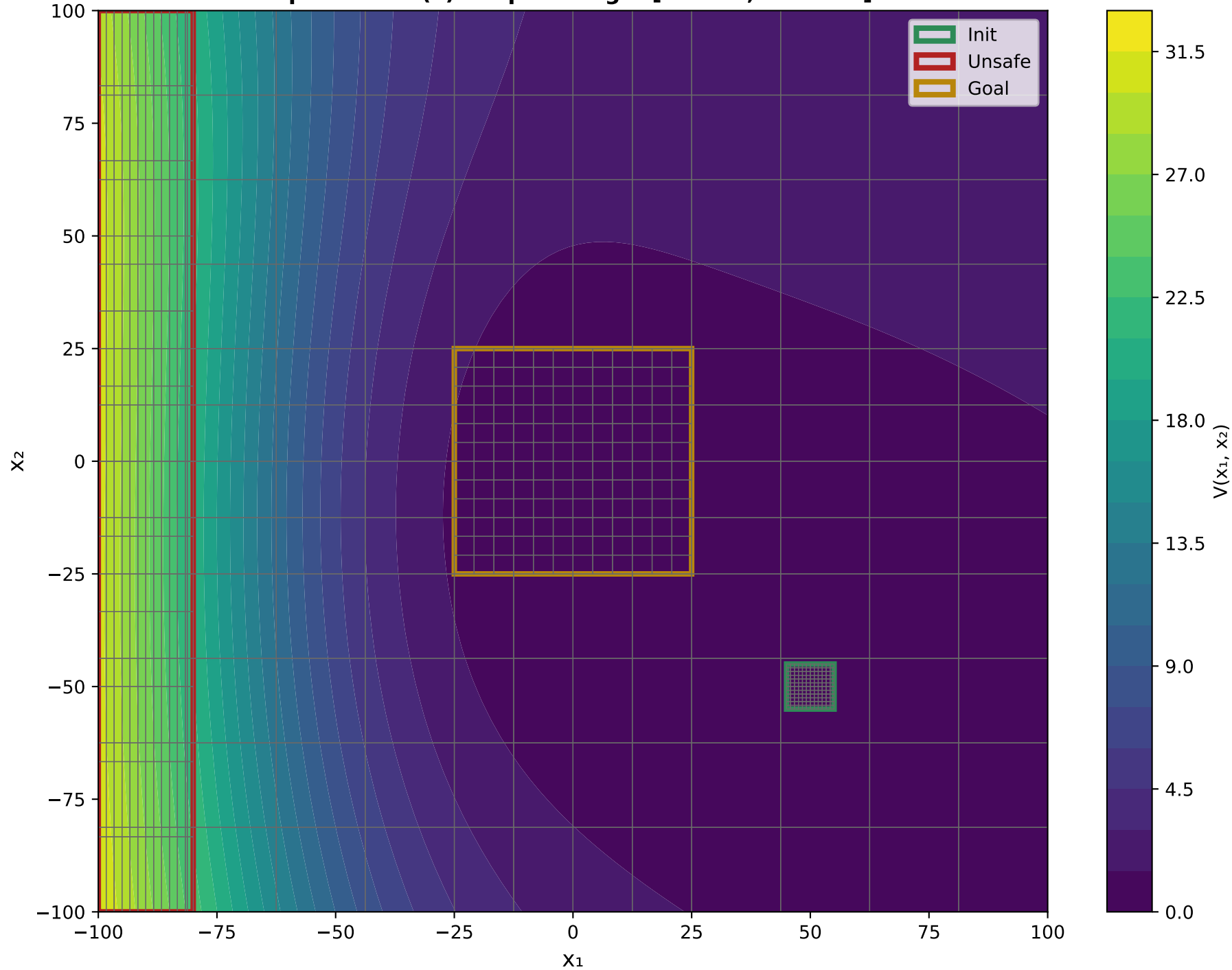
X 1 VS X 2 Epoch: 0 - V(x) Output Range: [0.1482, 31.5317]
