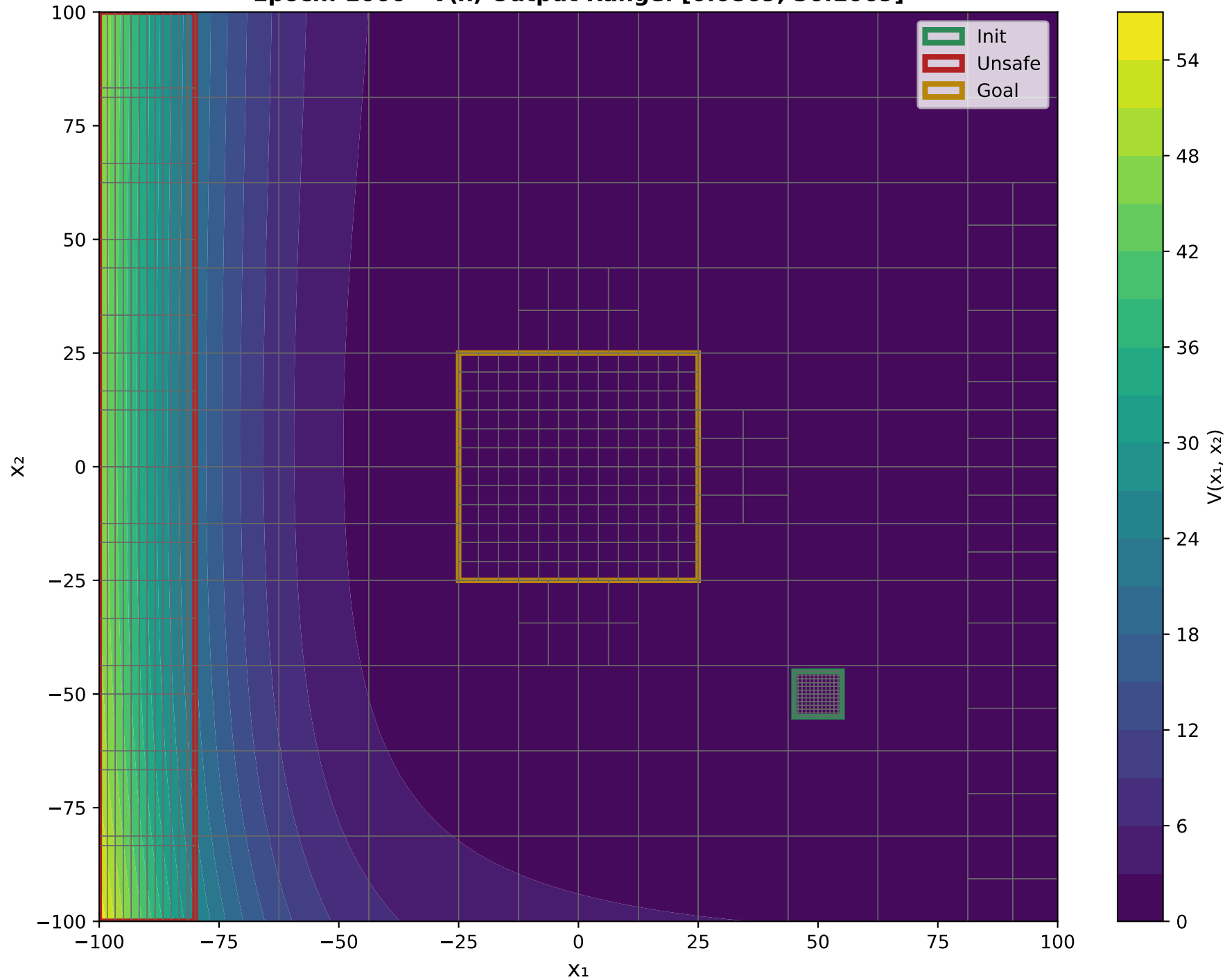
X 1 VS X 2 Epoch: 1000 - V(x) Output Range: [0.0869, 56.1069]
