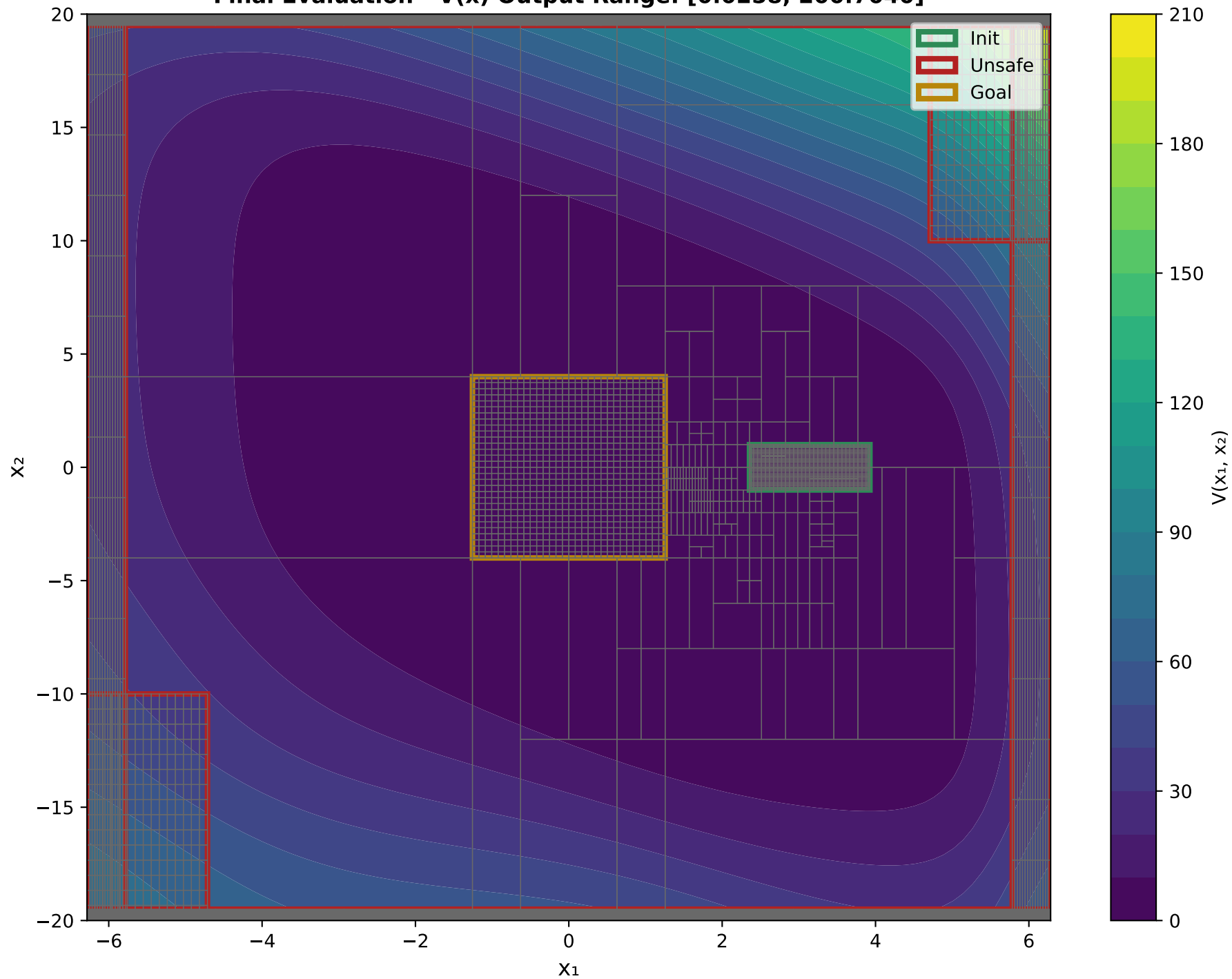
X 1 VS X 2 Final Evaluation - V(x) Output Range: [0.0258, 200.7040]
