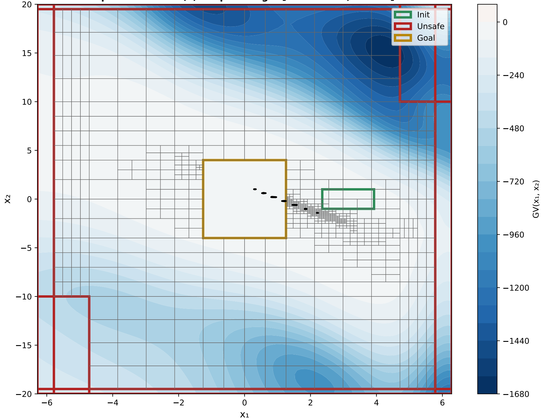
X 1 VS X 2 Epoch 2000 - GV(x) Output Range: [-1658.6360, 0.0541]
