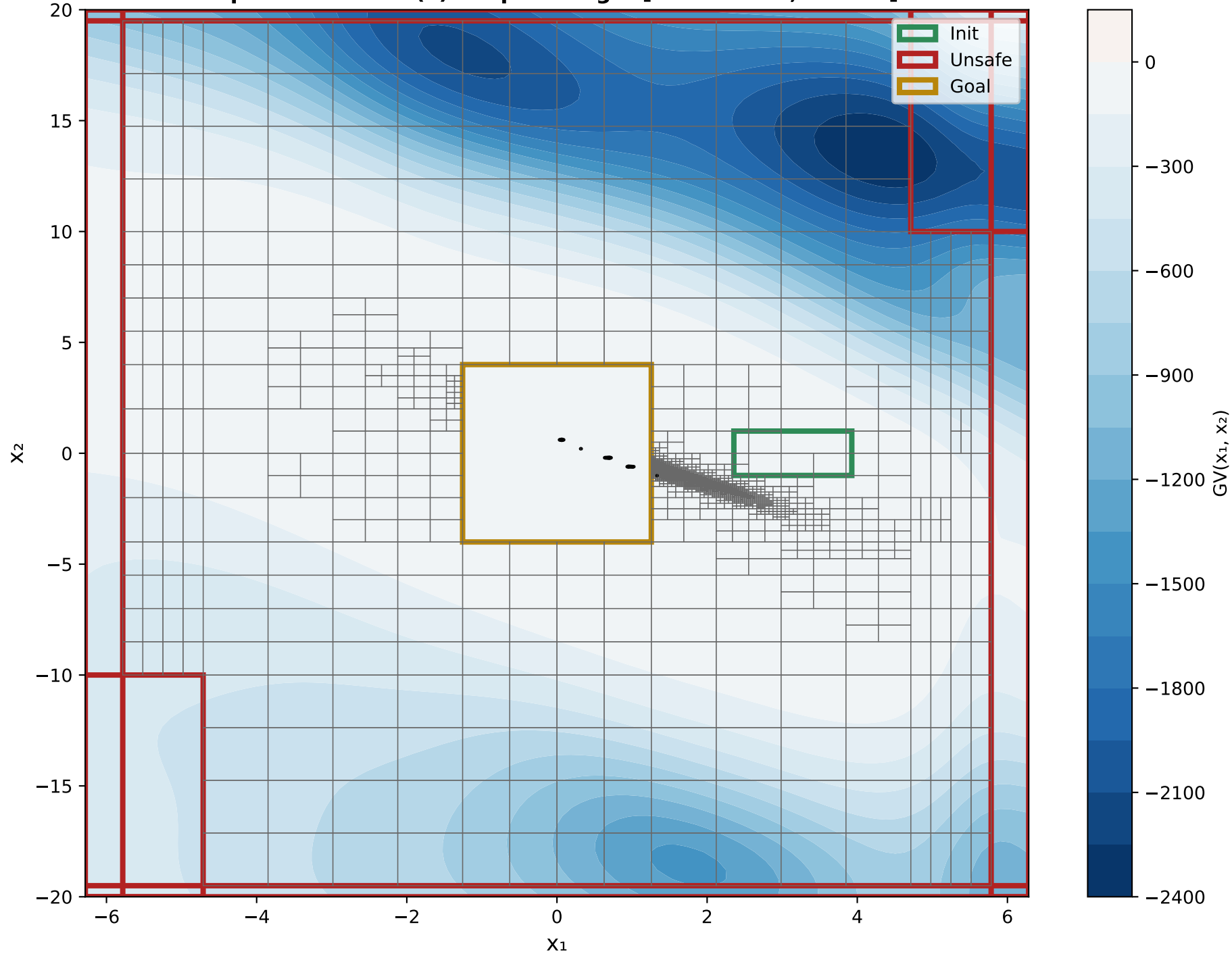
X 1 VS X 2 Epoch 4000 - GV(x) Output Range: [-2390.4197, 0.0235]
