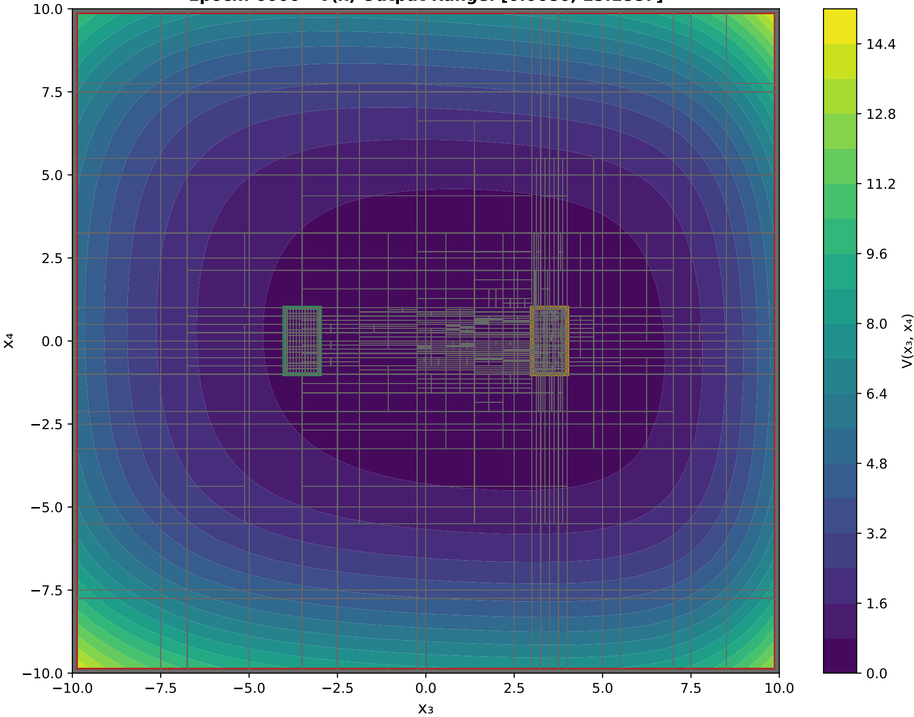
X 3 VS X 4 Epoch: 6000 - V(x) Output Range: [0.0680, 15.1887]
