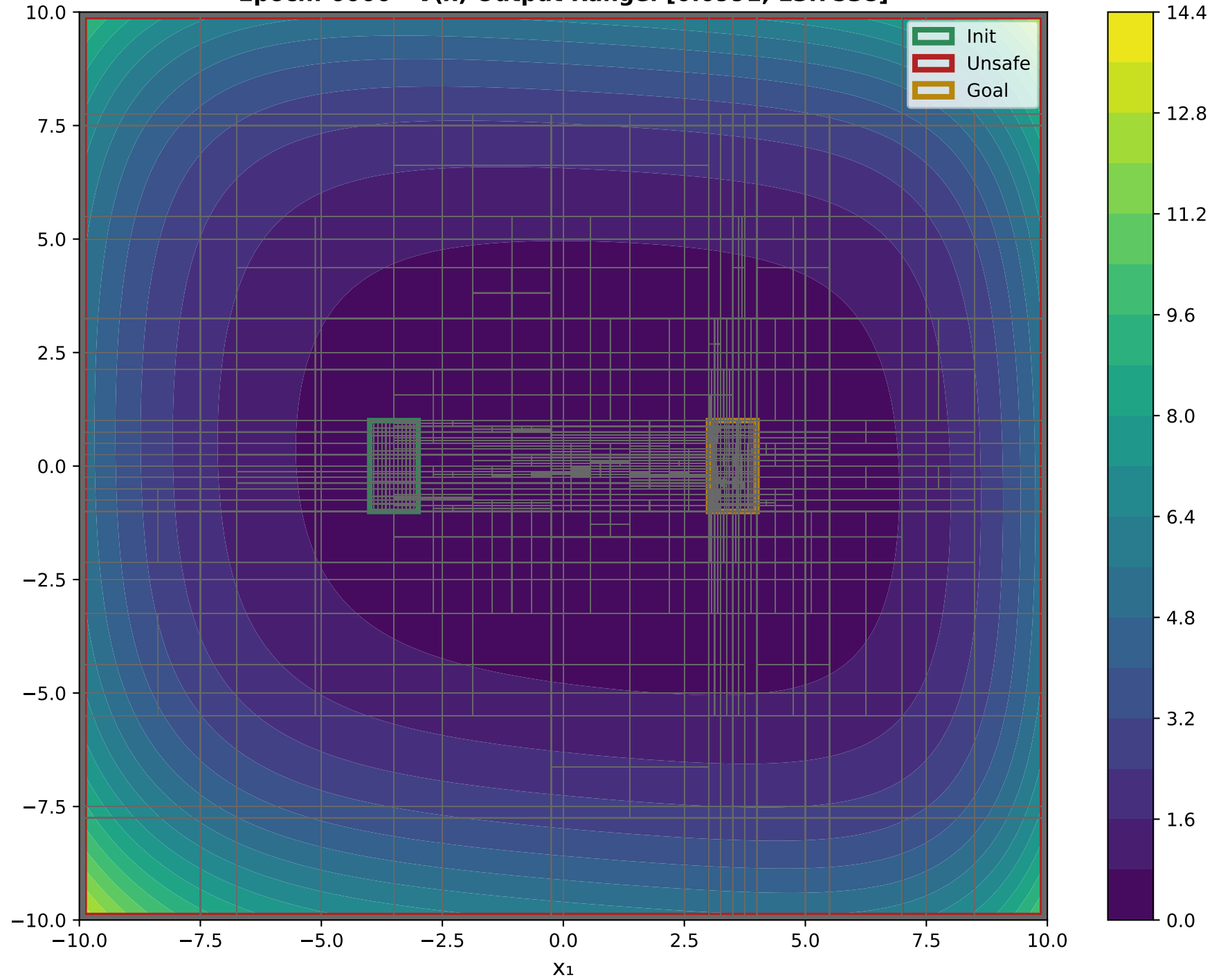
X 1 VS X 2 Epoch: 6000 - V(x) Output Range: [0.0991, 13.7538]
