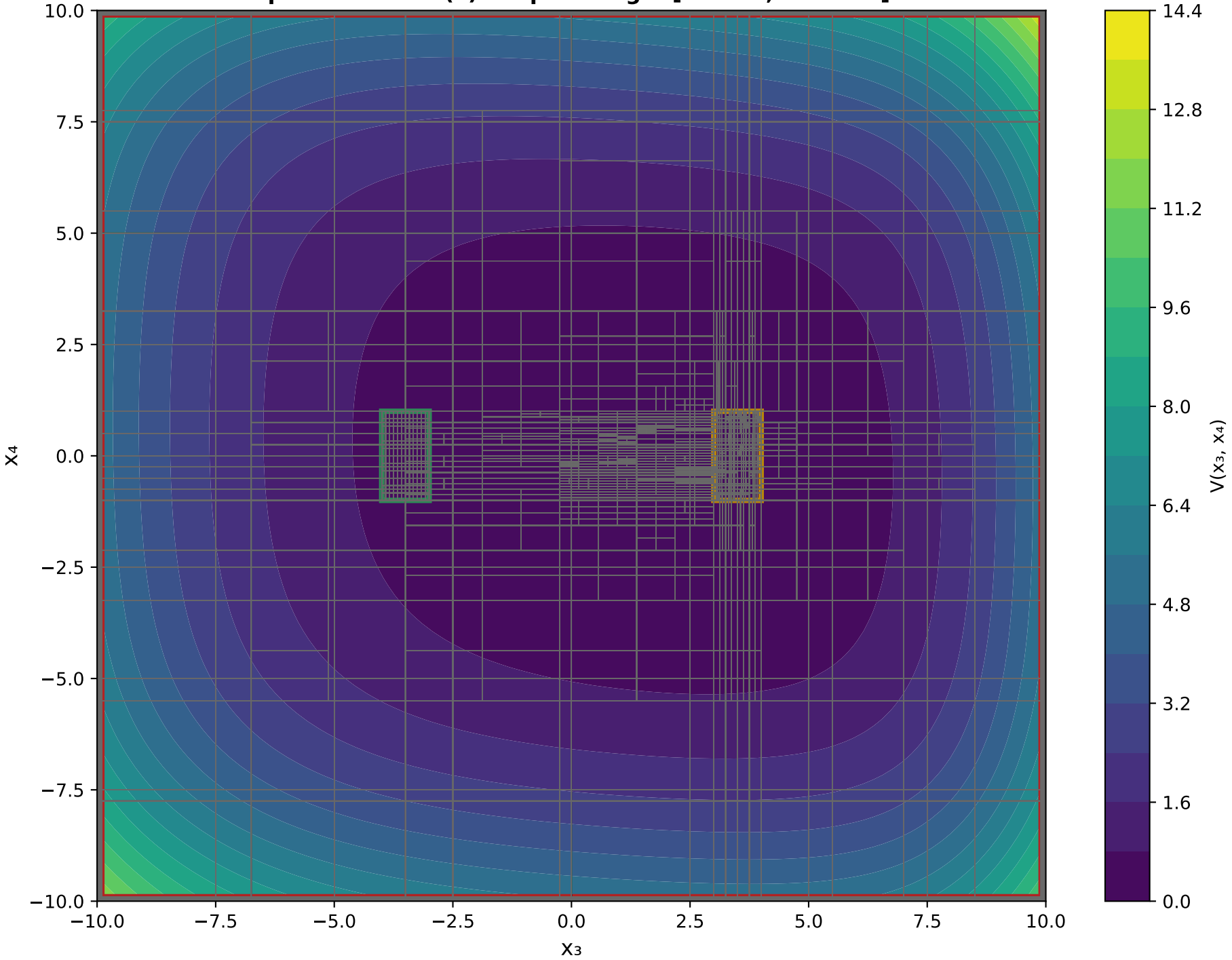
X3 VS X4 Epoch: 8000 - V(x) Output Range: [0.0534, 14.0073]
