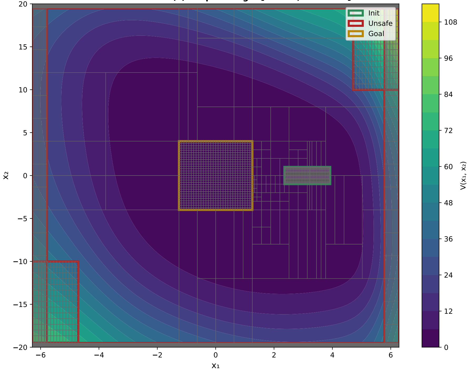
X 1 VS X 2 Final Evaluation - V(x) Output Range: [0.0326, 113.9951]
