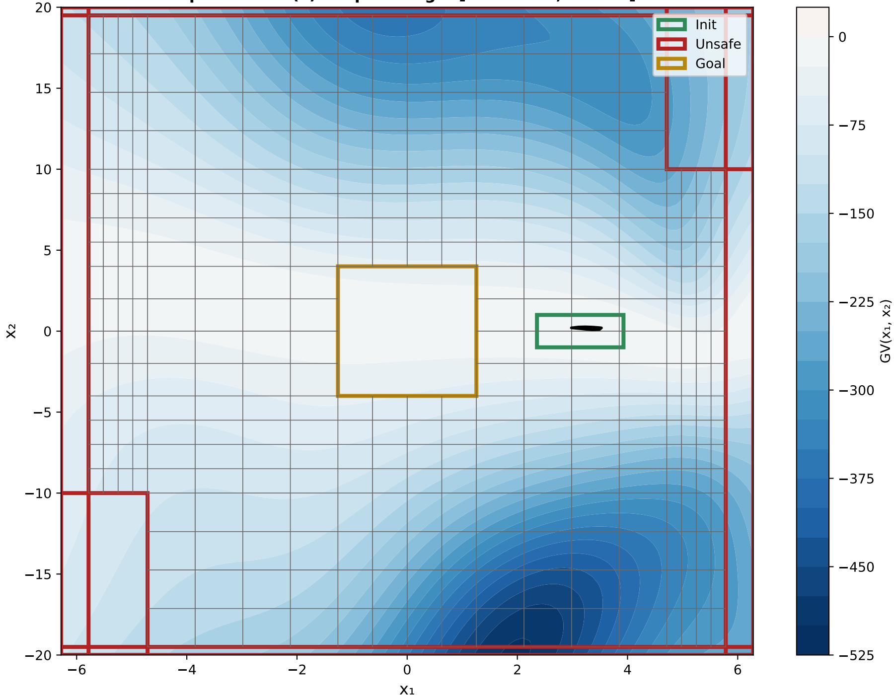
X 1 VS X 2 Epoch 0 - GV(x) Output Range: [-503.9997, 0.2622]
