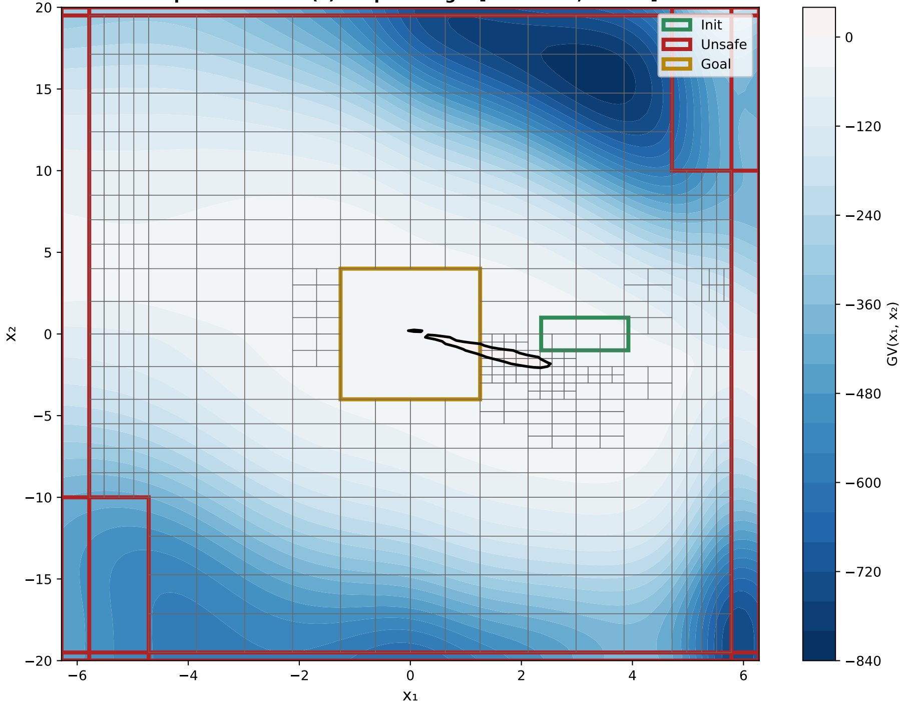
X 1 VS X 2 Epoch 1000 - GV(x) Output Range: [-829.5928, 0.2678]
