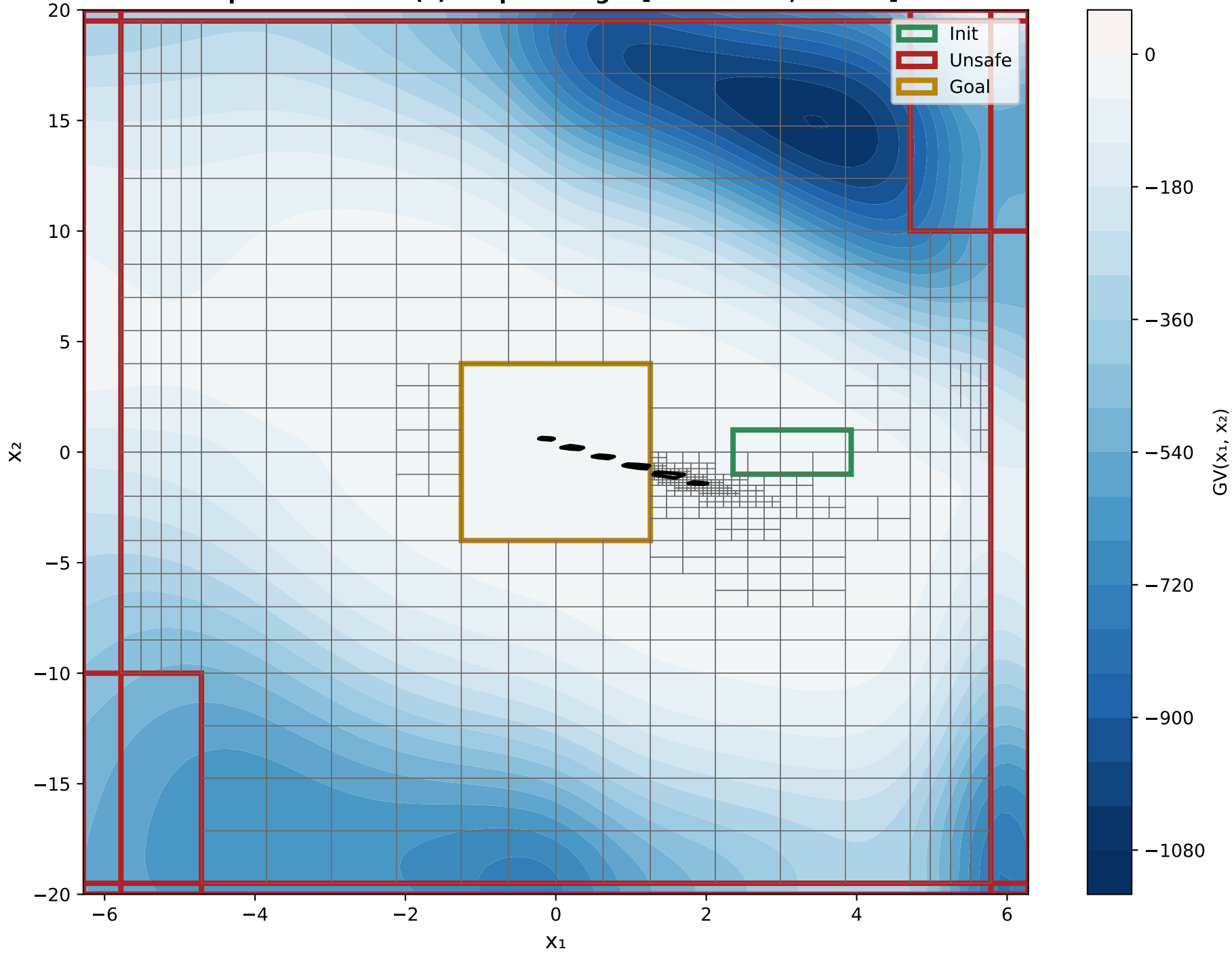
X 1 VS X 2 Epoch 2000 - GV(x) Output Range: [-1081.4907, 0.1355]
