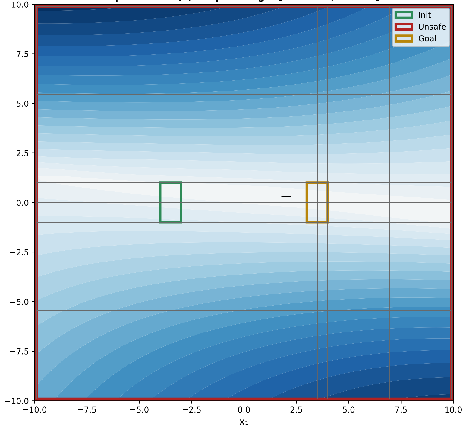
X 1 VS X 2 Epoch 0 - GV(x) Output Range: [-51.1727, 0.0140]
