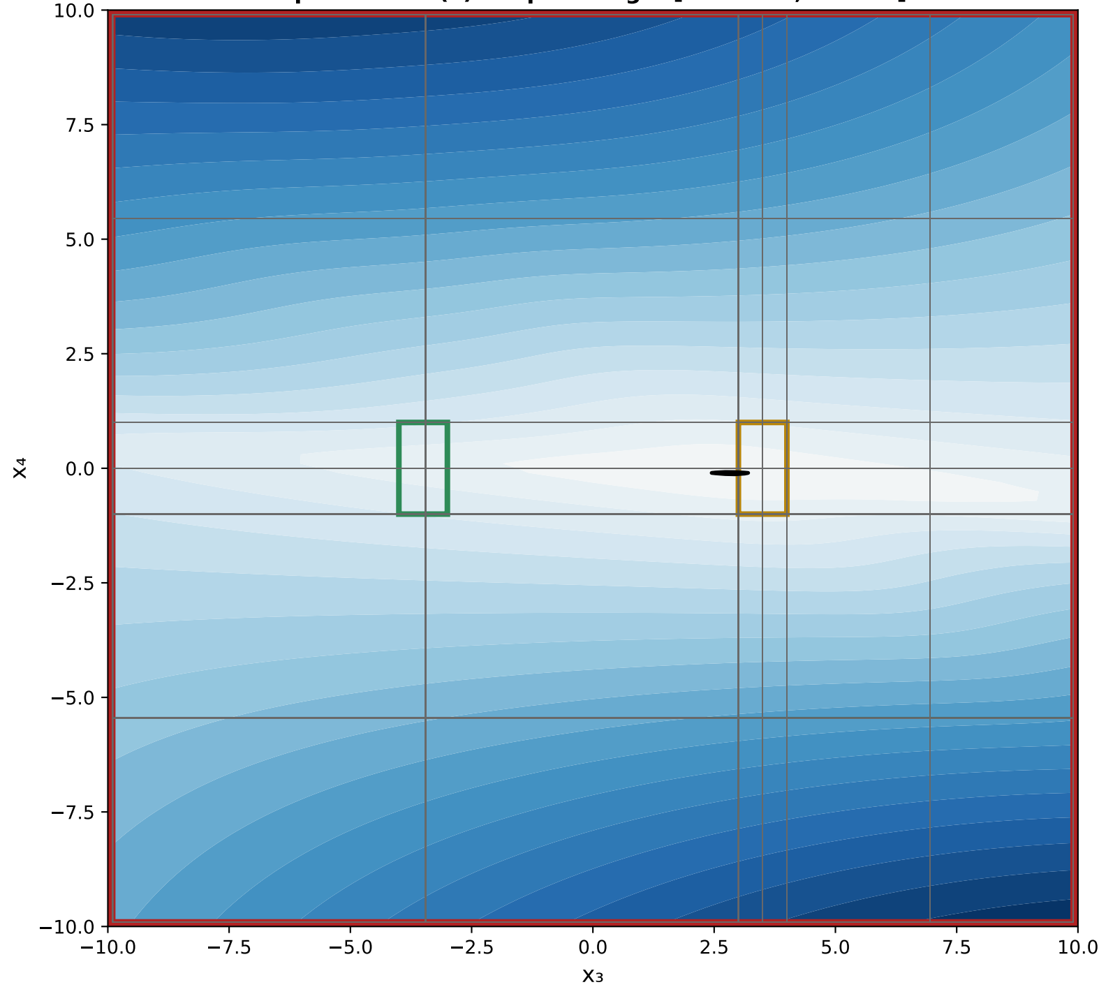
X 3 VS X 4 Epoch 0 - GV(x) Output Range: [-47.2102, 0.0564]
