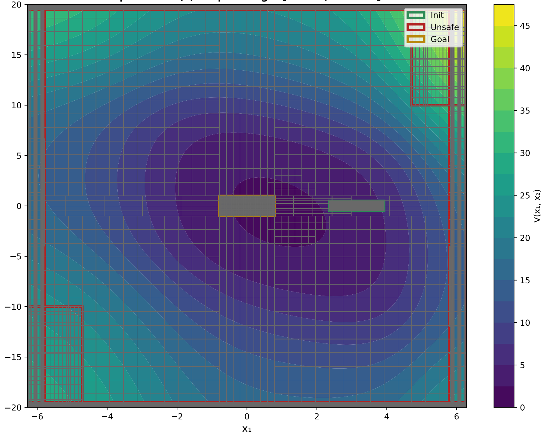
X 1 VS X 2 Epoch: 0 - V(x) Output Range: [2.1119, 47.0791]
