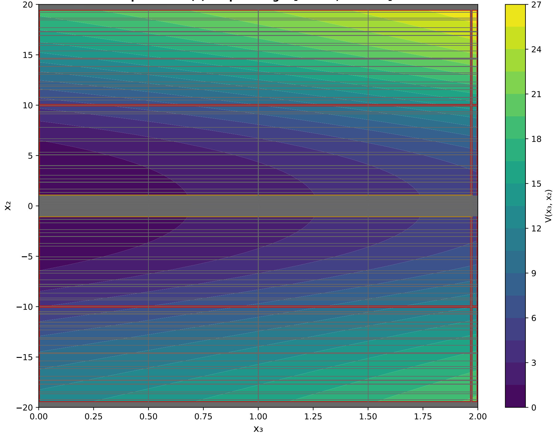
X 3 VS X 2 Epoch: 0 - V(x) Output Range: [0.1001, 26.9413]
