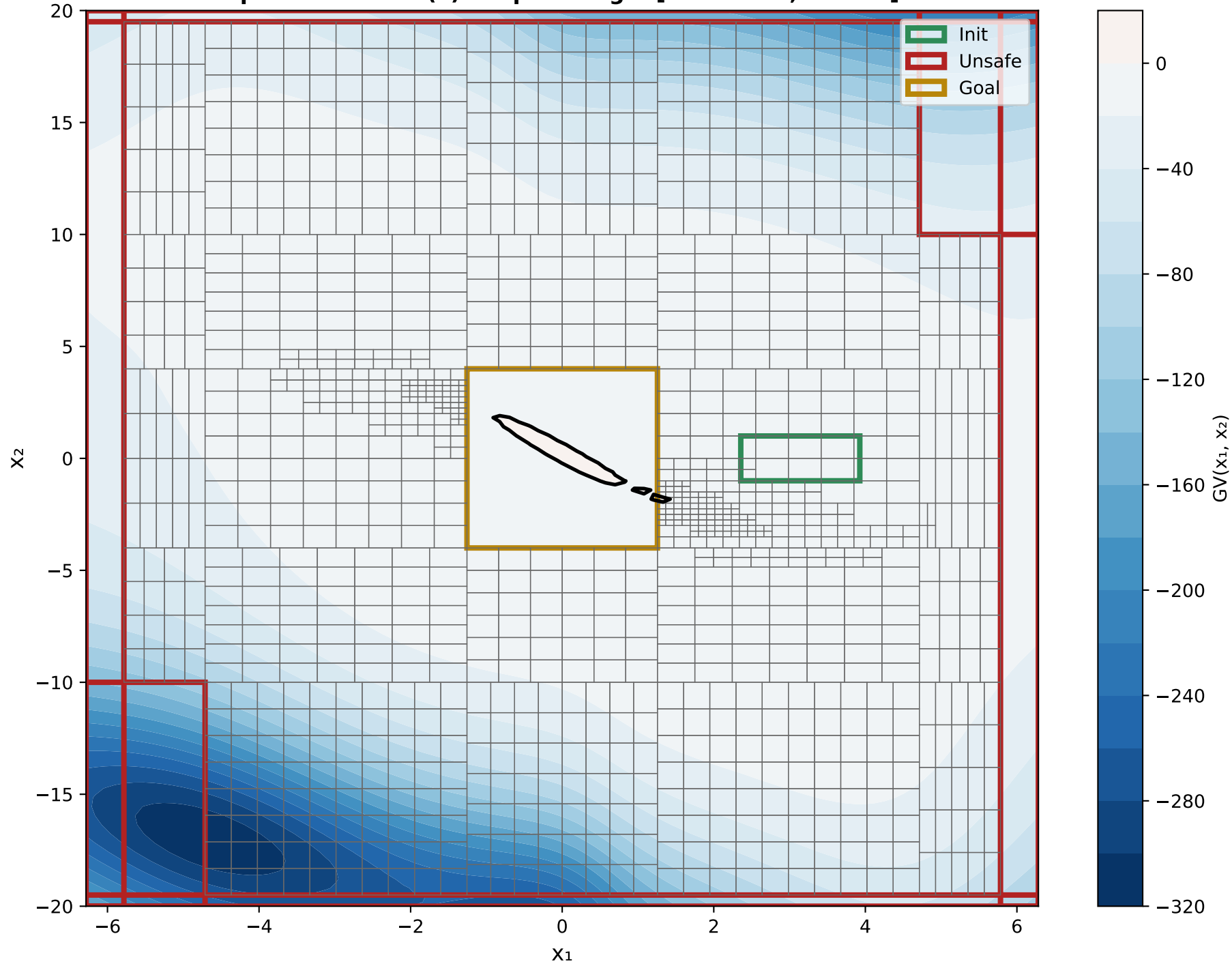
X 1 VS X 2 Epoch 1000 - GV(x) Output Range: [-315.3753, 0.1343]
