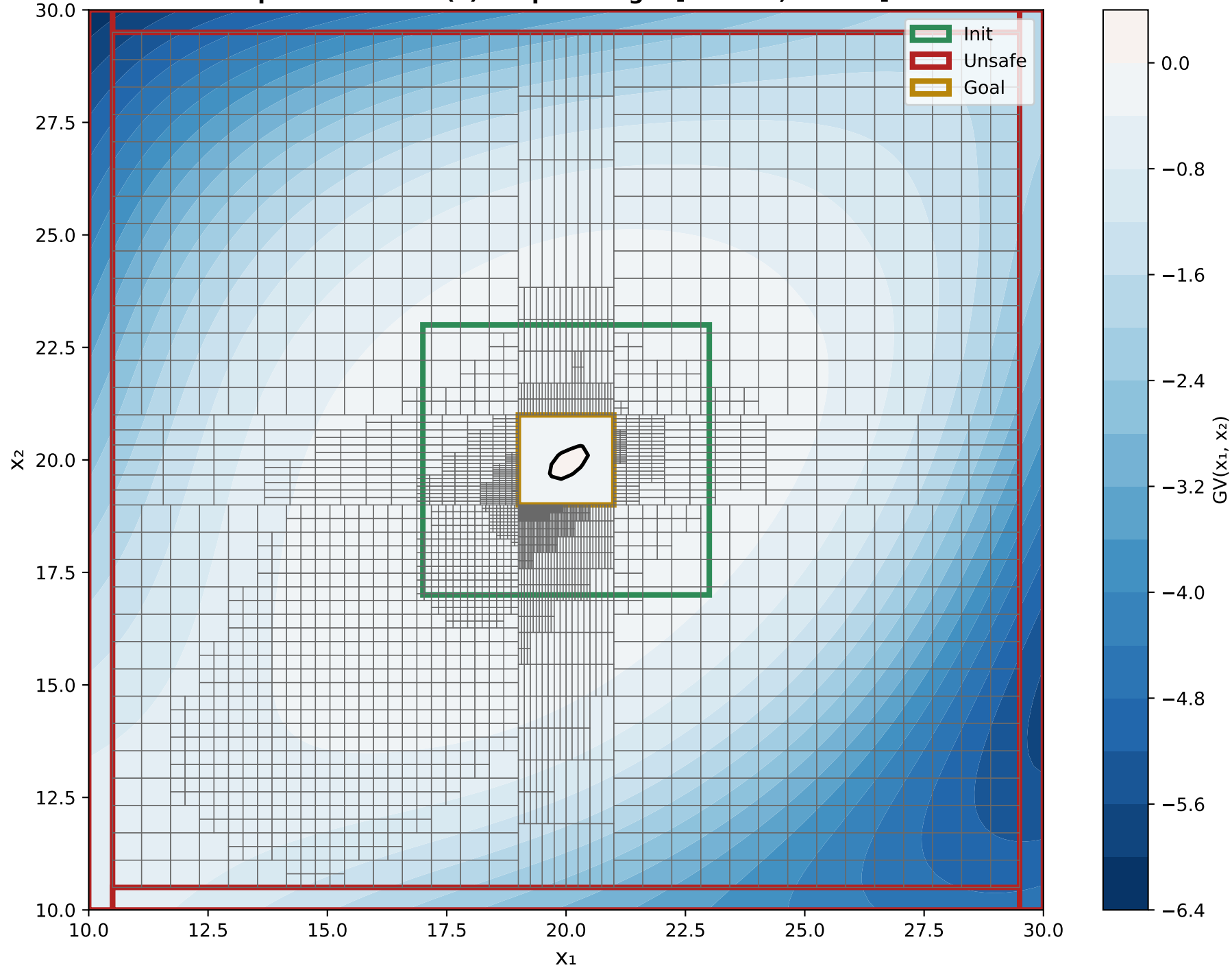
X 1 VS X 2 Epoch 3000 - GV(x) Output Range: [-6.3167, 0.0009]
