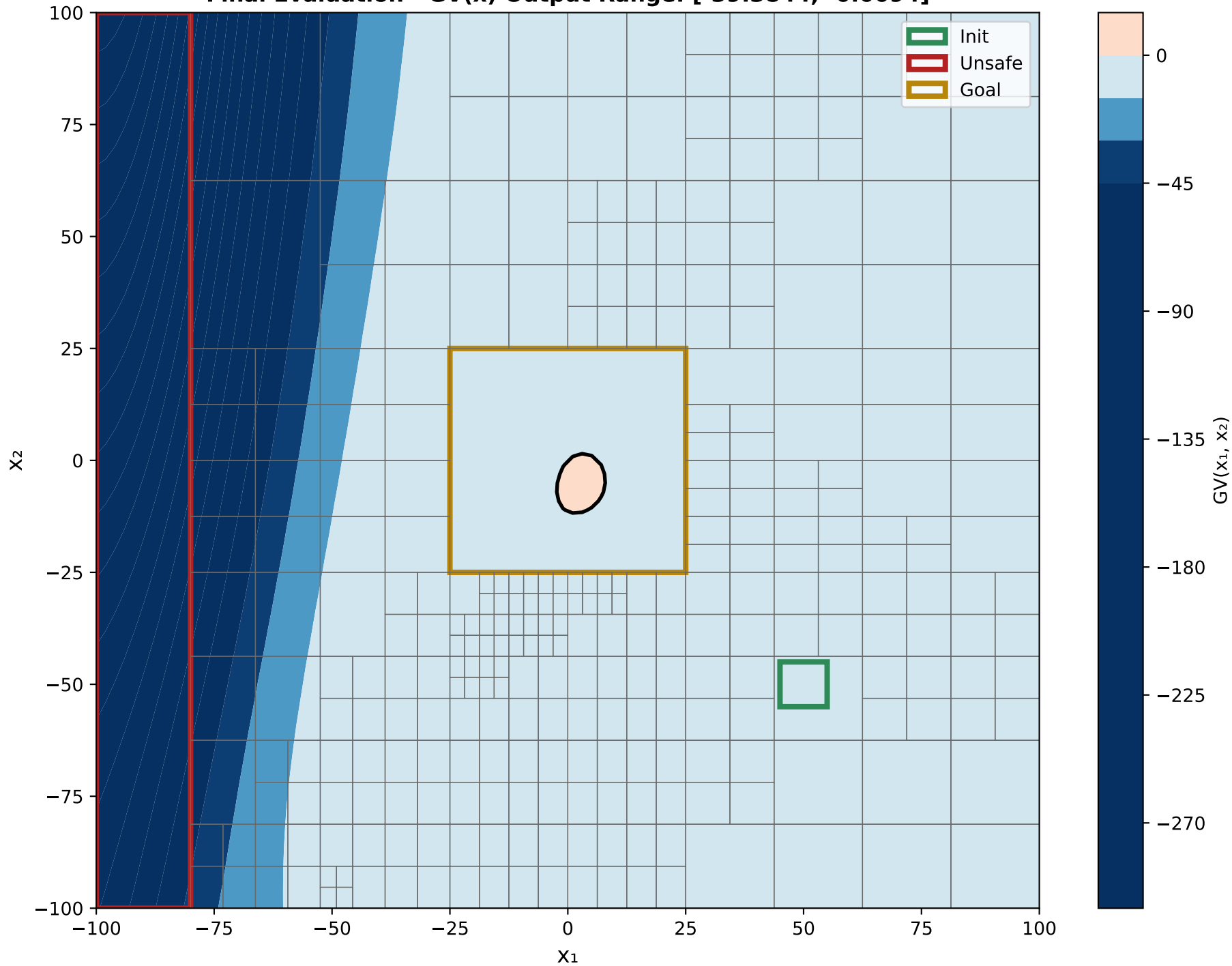
X 1 VS X 2 Final Evaluation - GV(x) Output Range: [-39.3844, -0.0094]
