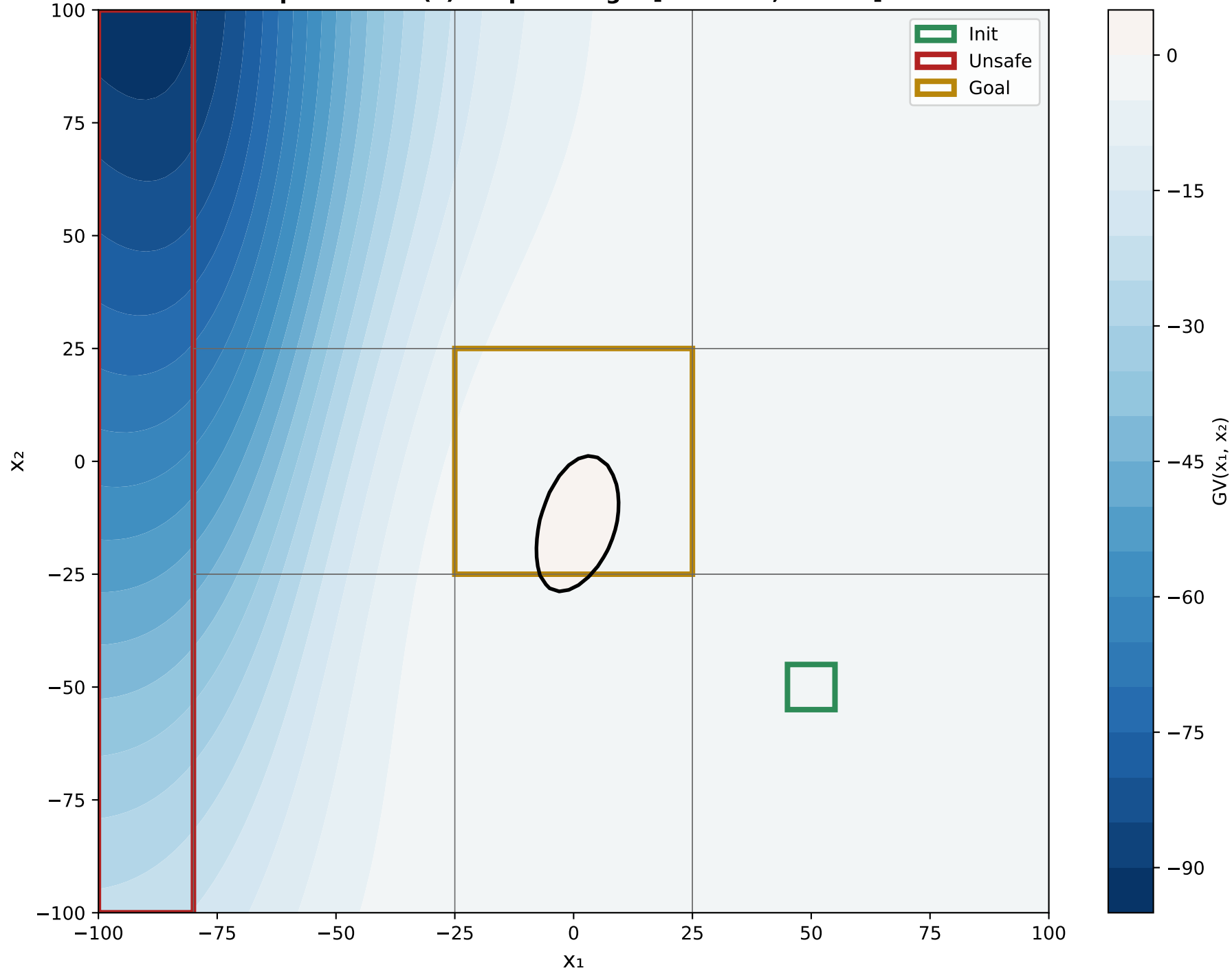
X 1 VS X 2 Epoch 0 - GV(x) Output Range: [-94.3473, 0.1683]
