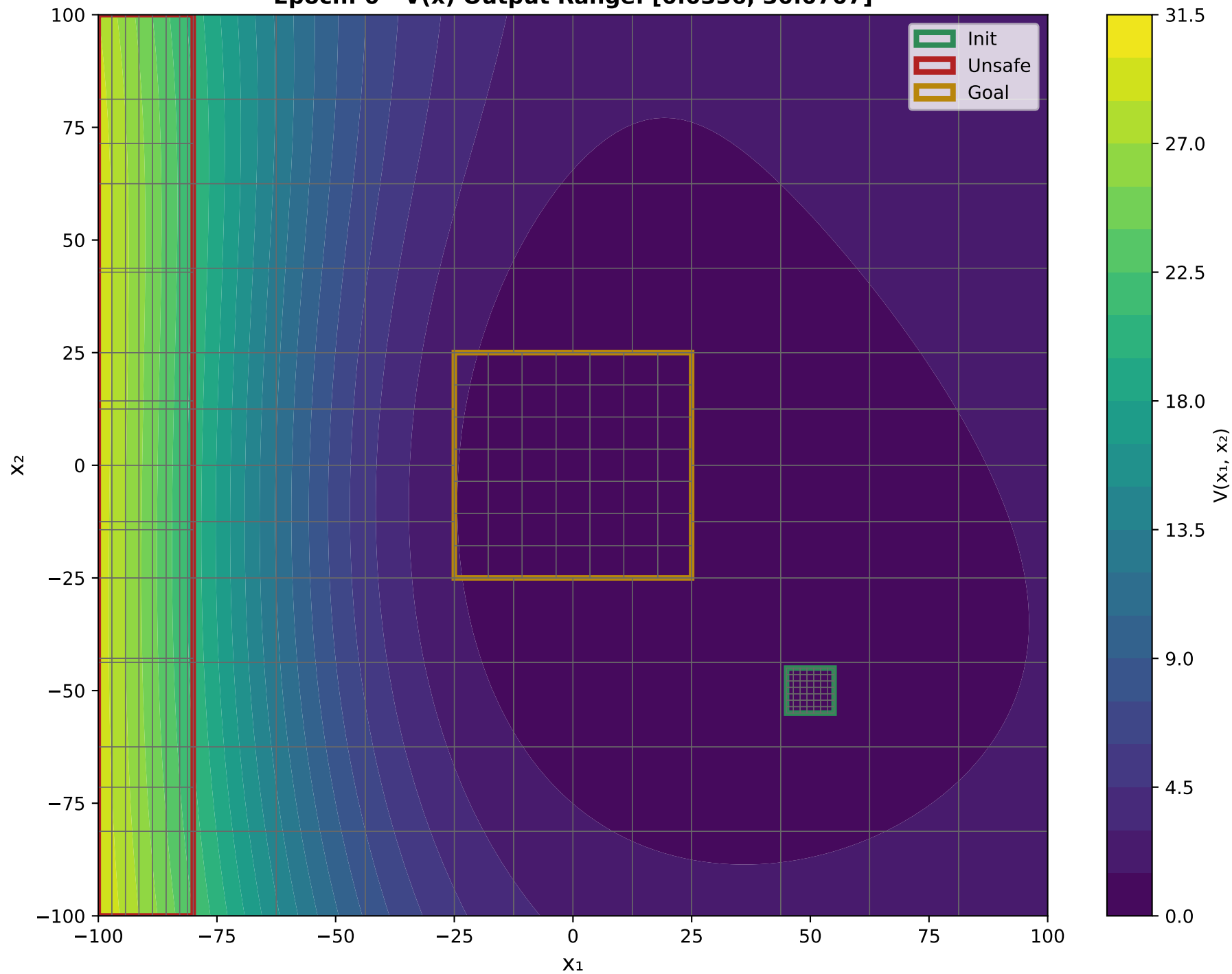
X 1 VS X 2 Epoch: 0 - V(x) Output Range: [0.0336, 30.0707]
