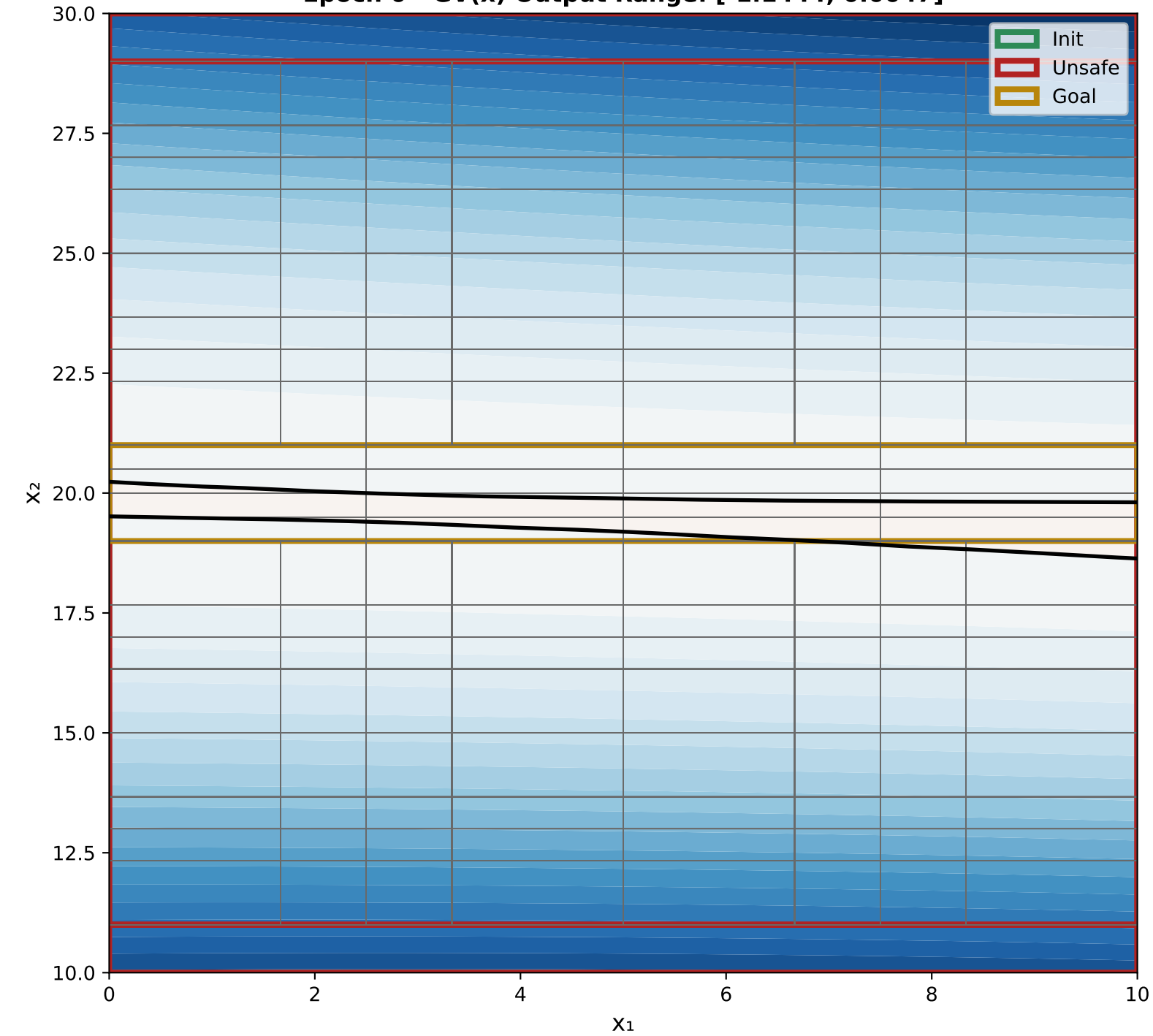
X 1 VS X 2 Epoch 0 - GV(x) Output Range: [-1.1444, 0.0047]
