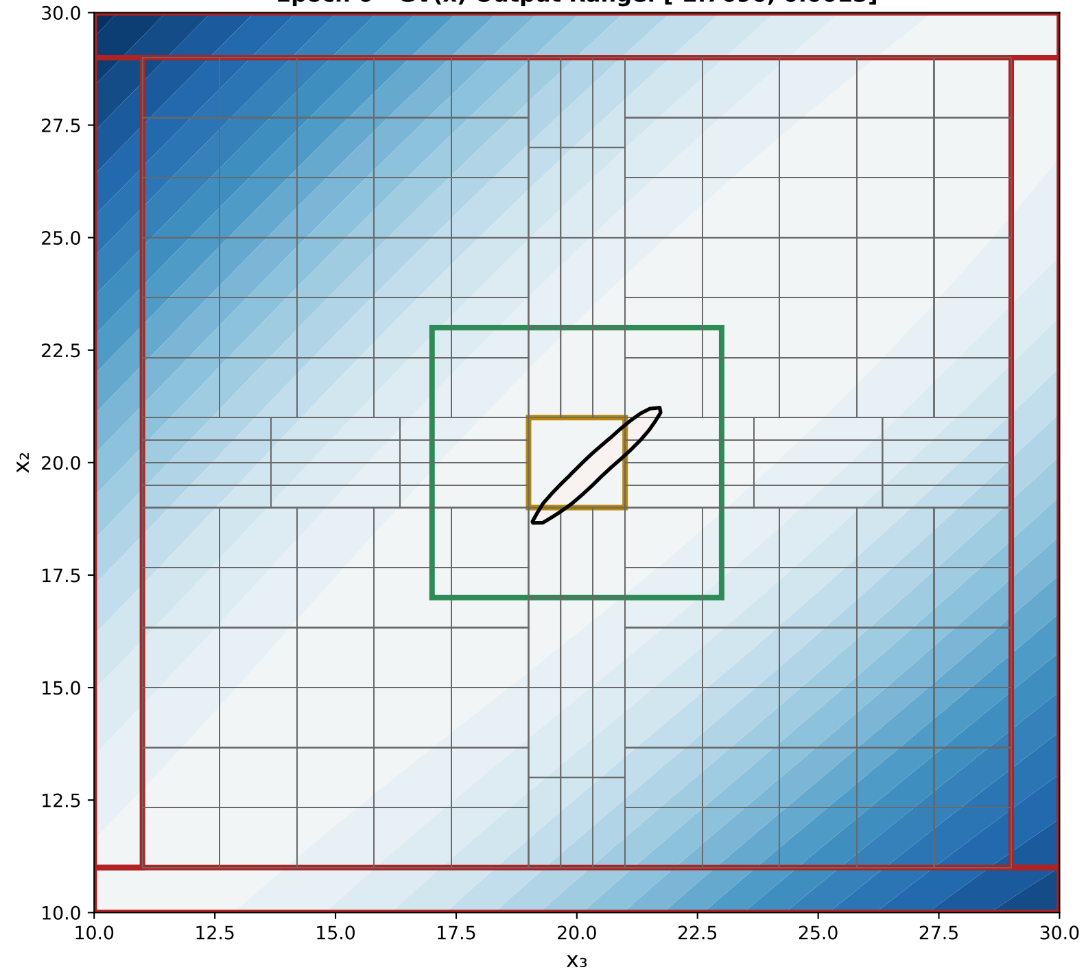
X 3 VS X 2 Epoch 0 - GV(x) Output Range: [-2.7690, 0.0015]
