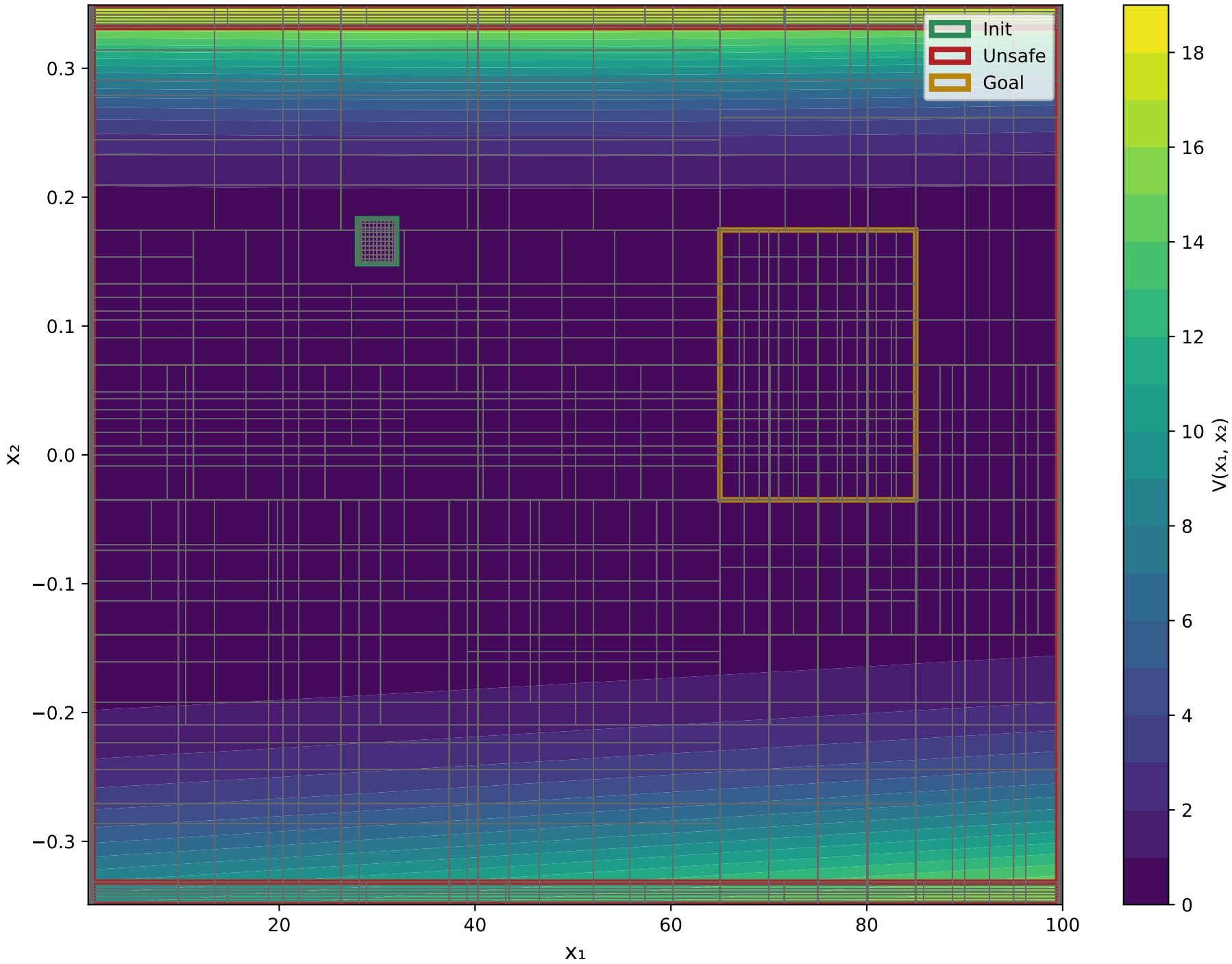
X 1 VS X 2 Epoch: 1000 - V(x) Output Range: [0.0910, 18.5904]
