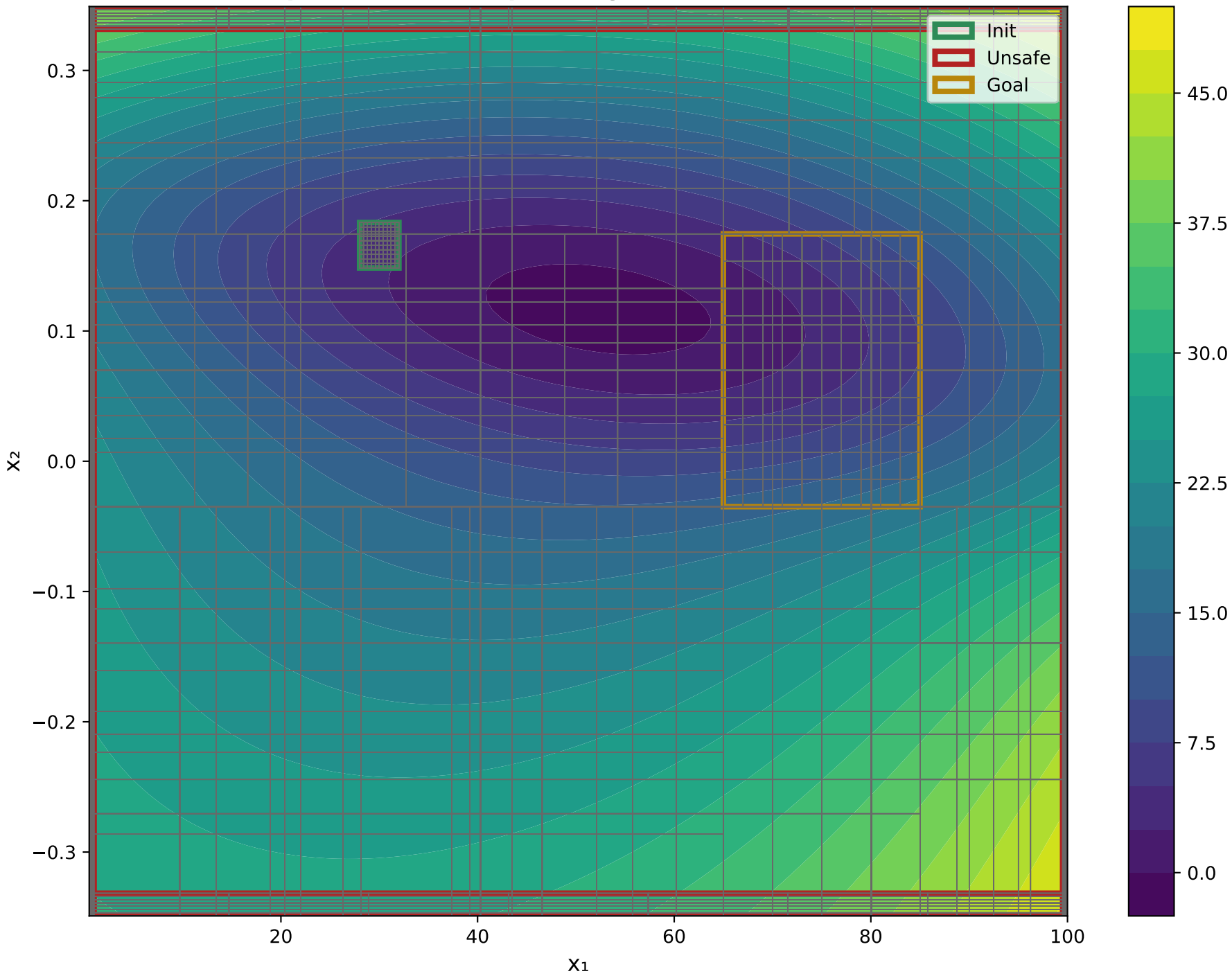
X 1 VS X 2 Epoch: 0 - V(x) Output Range: [-1.0435, 48.1313]
