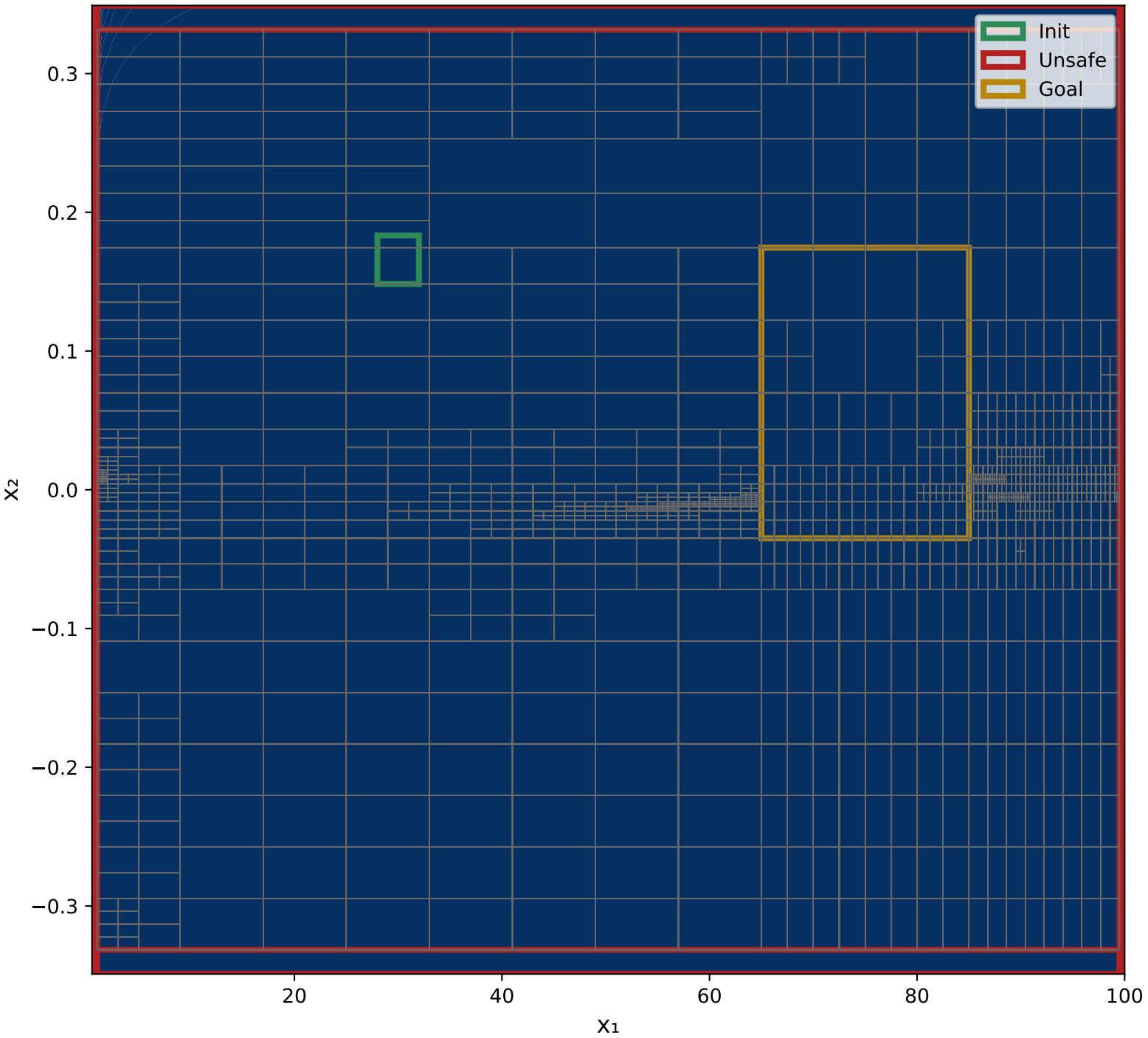
X 1 VS X 2 Final Evaluation - GV(x) Output Range: [-52.0204, -0.0000]
