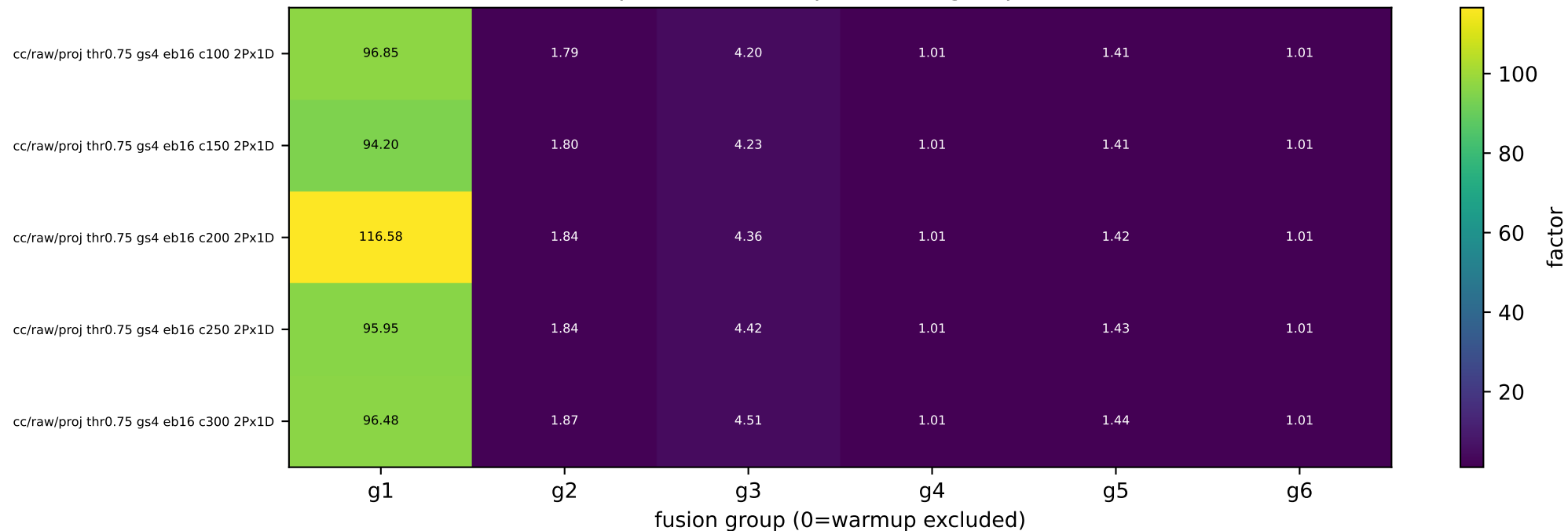
BFF compression factor per fusion group (× smaller)
