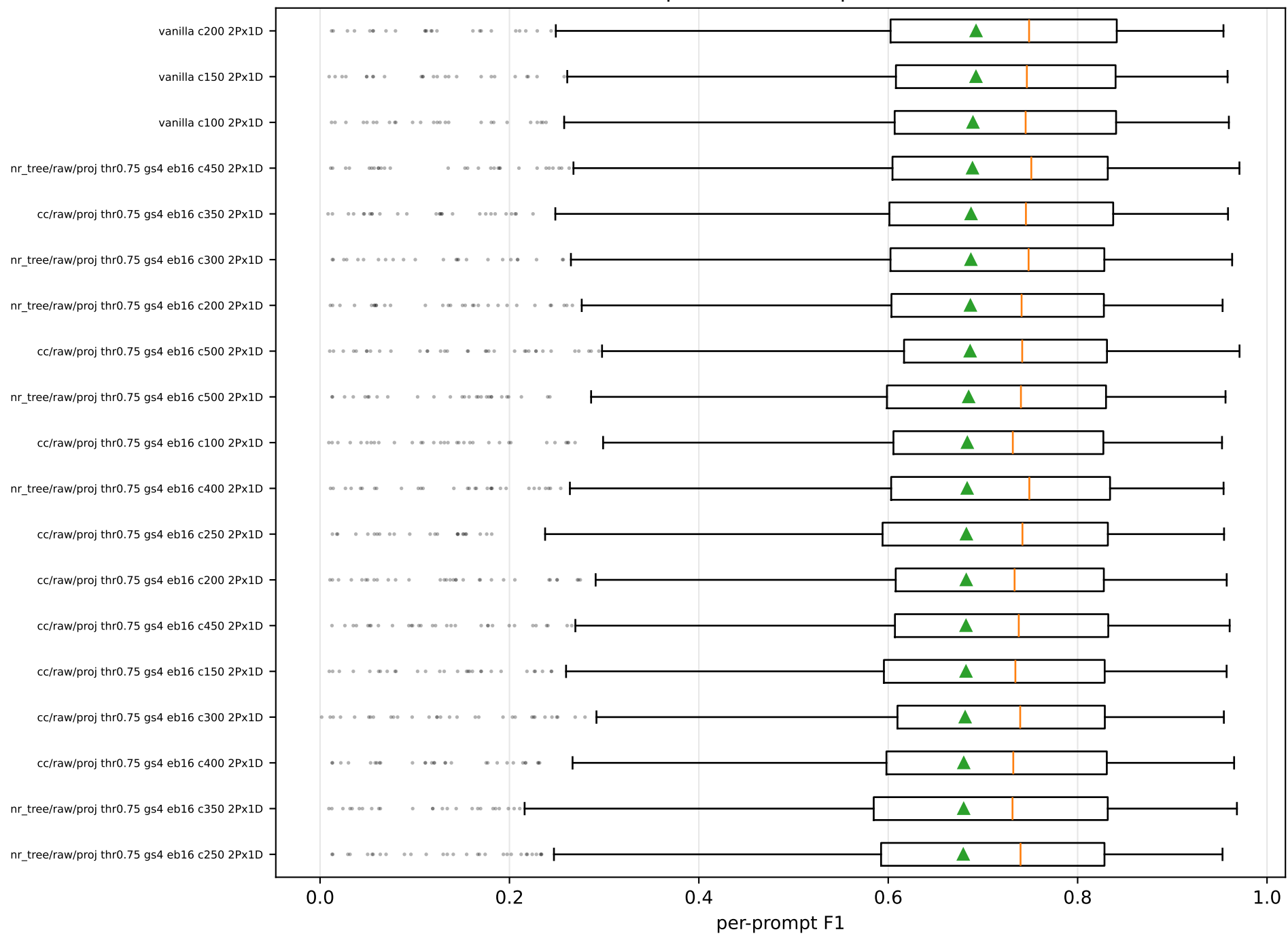
F1 distribution per run (box = quartiles, ▲ = mean)
