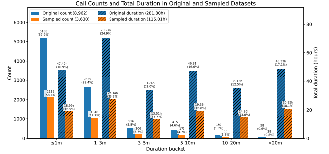
Figure 1: Comparison between the original conversational dataset and the sampled dataset across call duration buckets.
