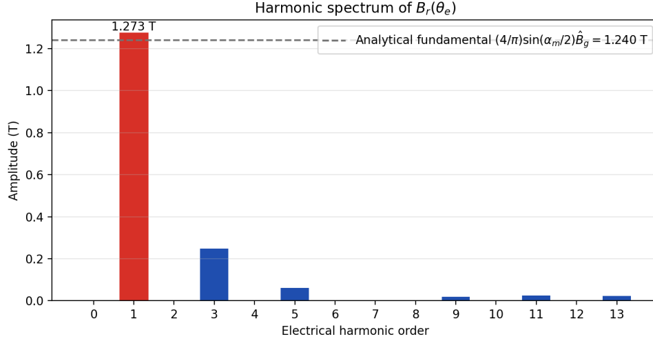
Figure 13: Harmonic spectrum of B_r(\theta_e) .
