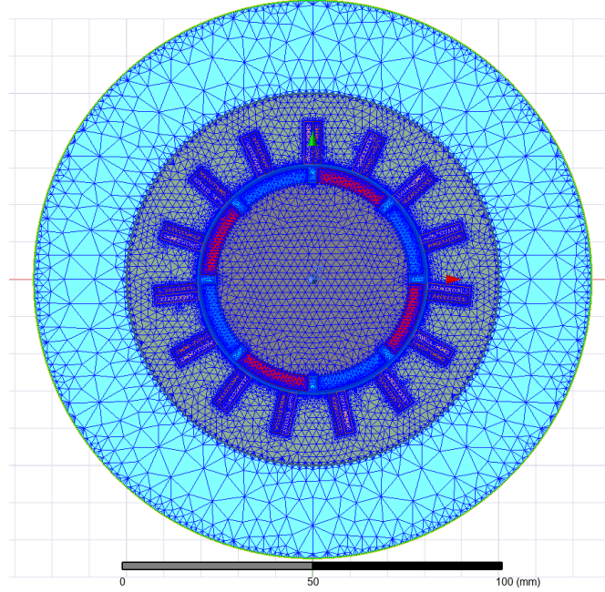
Figure 9: Final adapted mesh.
