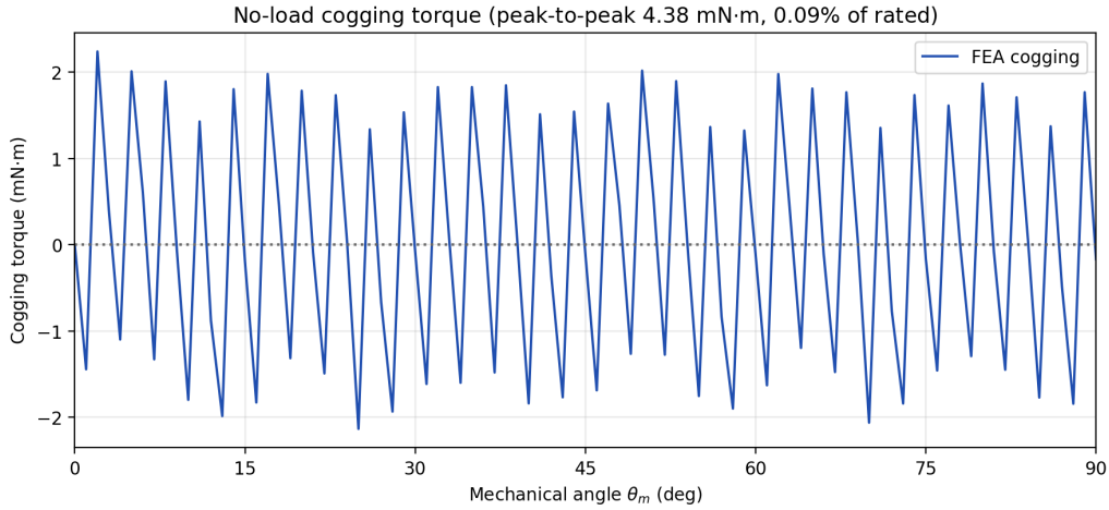
Figure 17: No-load cogging torque vs. rotor angle.
