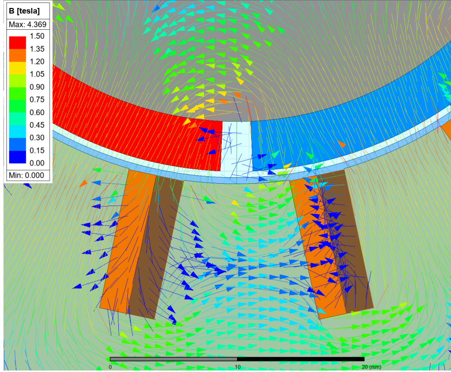
Figure 16: Tooth-tip leakage.
