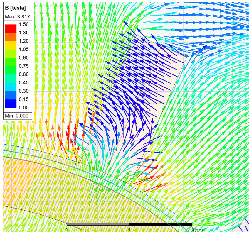
Figure 15: In-slot leakage.
