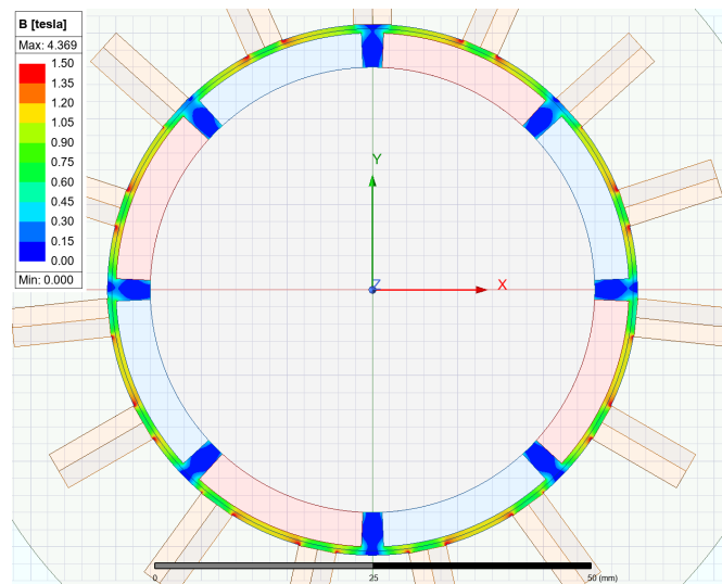
Figure 11: |\mathbf{B}| across the air-gap.
