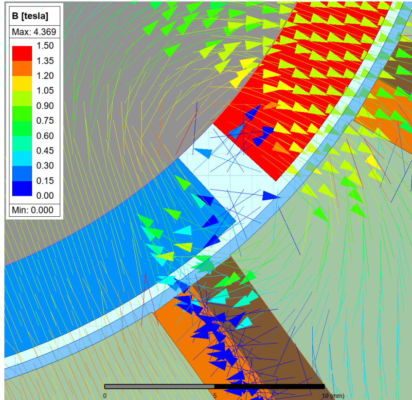
Figure 14: Magnet-to-magnet leakage.
