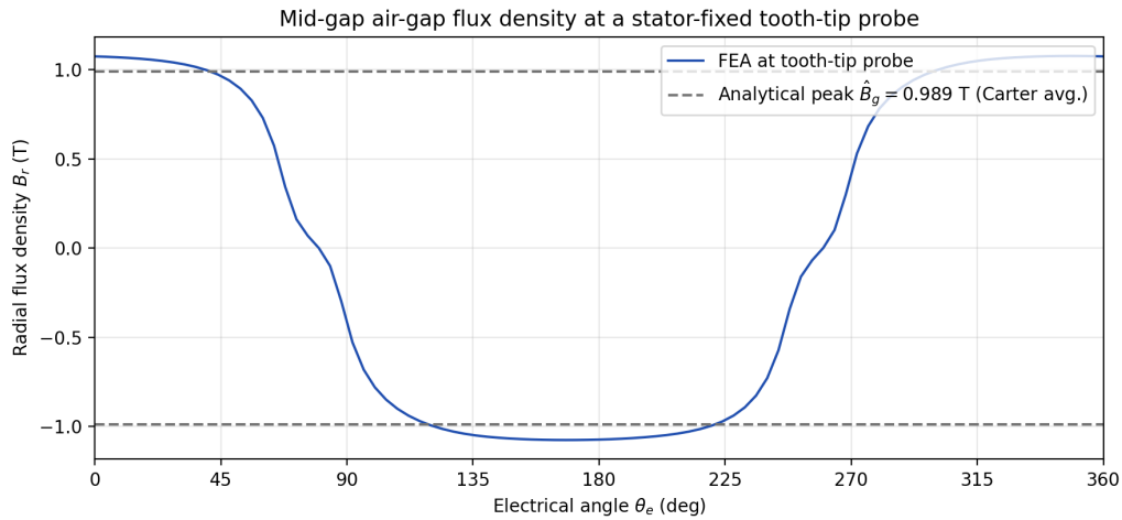
Figure 12: Mid-gap B_r at the tooth-tip probe vs. electrical angle.
