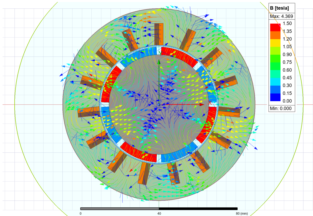
Figure 10: No-load flux density vectors over the full cross-section.
