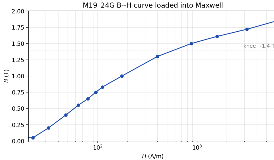
Figure 8: Imported M19_24G B–H curve.
