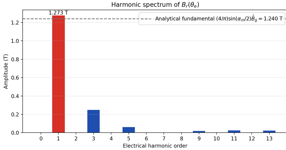
Figure 12: Harmonic spectrum of B_r(\theta_e) .
