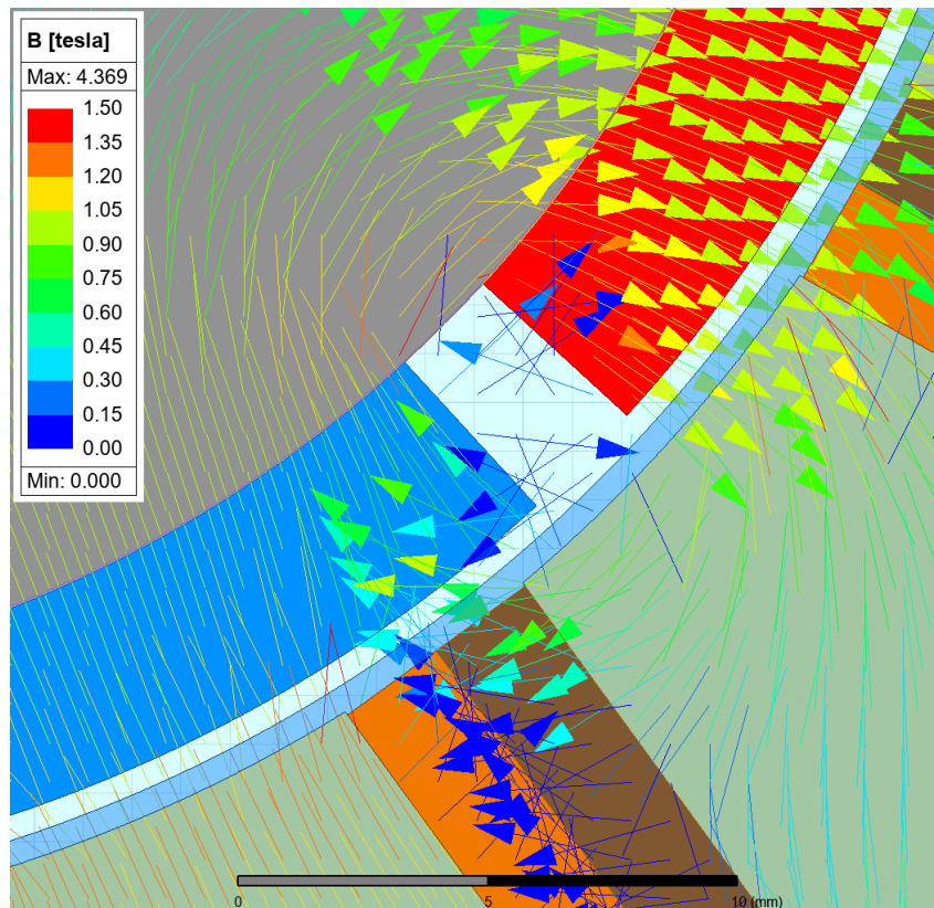
Figure 13: Magnet-to-magnet leakage.
