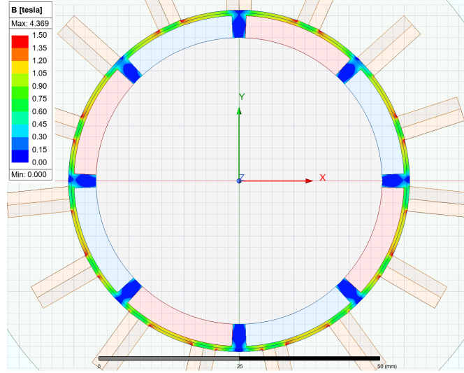
Figure 10: |\mathbf{B}| across the air-gap.
