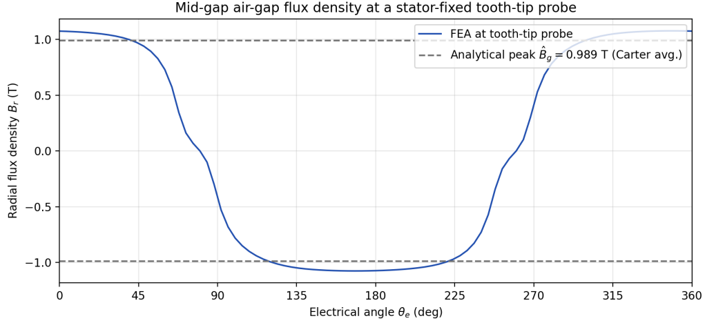
Figure 11: Mid-gap B_r at the tooth-tip probe vs. electrical angle.
