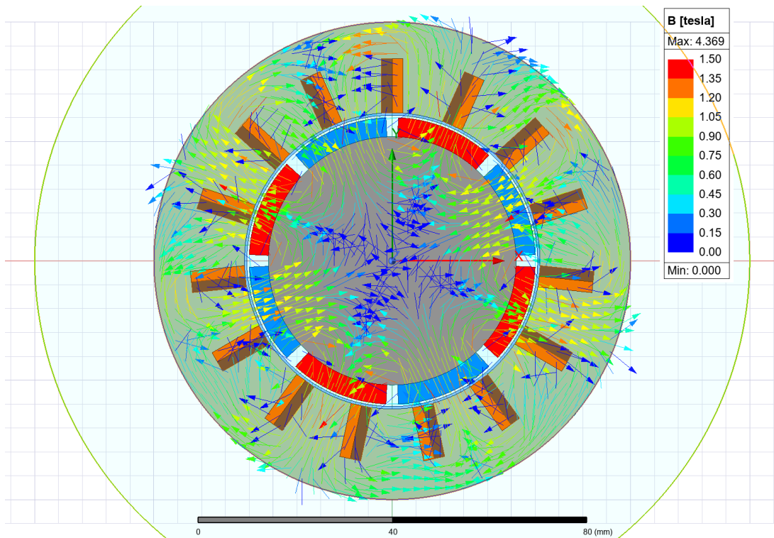
Figure 9: No-load flux density vectors over the full cross-section.
