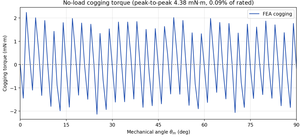
Figure 16: No-load cogging torque vs. rotor angle.
