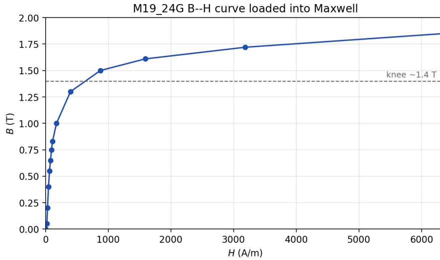
Figure 8: Imported M19_24G B–H curve.
