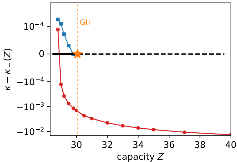
(b) offsets from the Hopf curve
