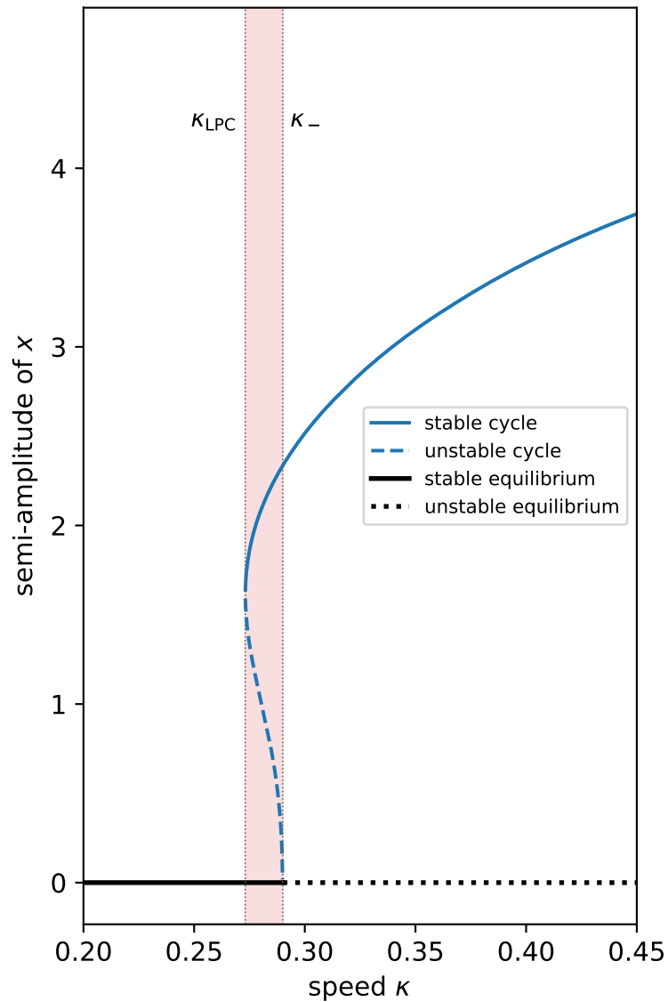
(c) Z = 45 : hysteresis in \kappa
