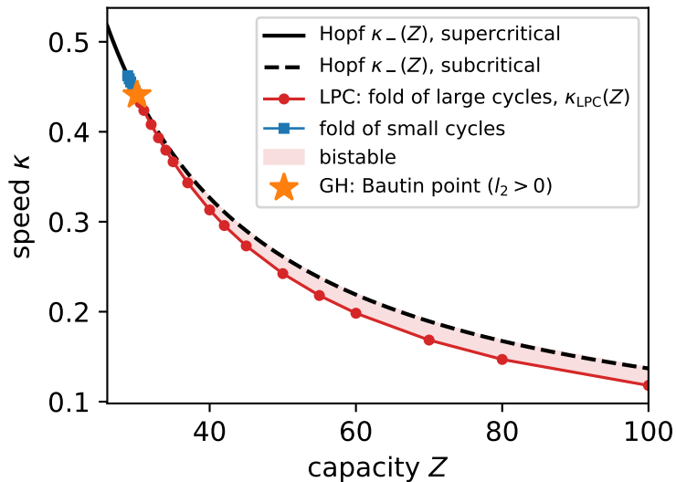
(a) lower window edge in the (Z, \kappa) plane
