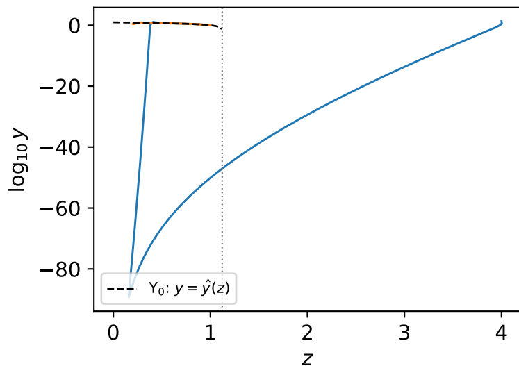
(a) \kappa = 0.05 : delayed passage through z = \zeta
