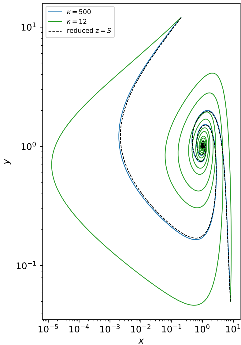
(c) fast adjustment versus the reduced system
