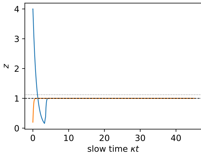
(b) z(t) ; dashed: z_* ; dotted: \zeta
