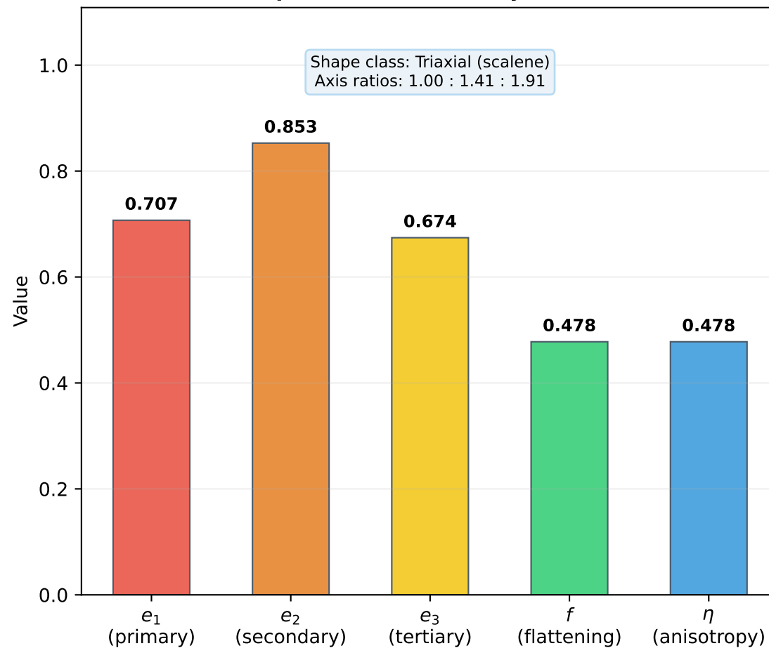
(b) Eccentricity Measures (0 = sphere, 1 = maximally deformed)
