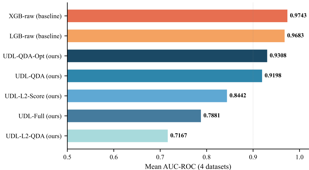
Mean AUC-ROC Across 4 ODDS Benchmarks (UDL Standalone vs Supervised Baselines)
