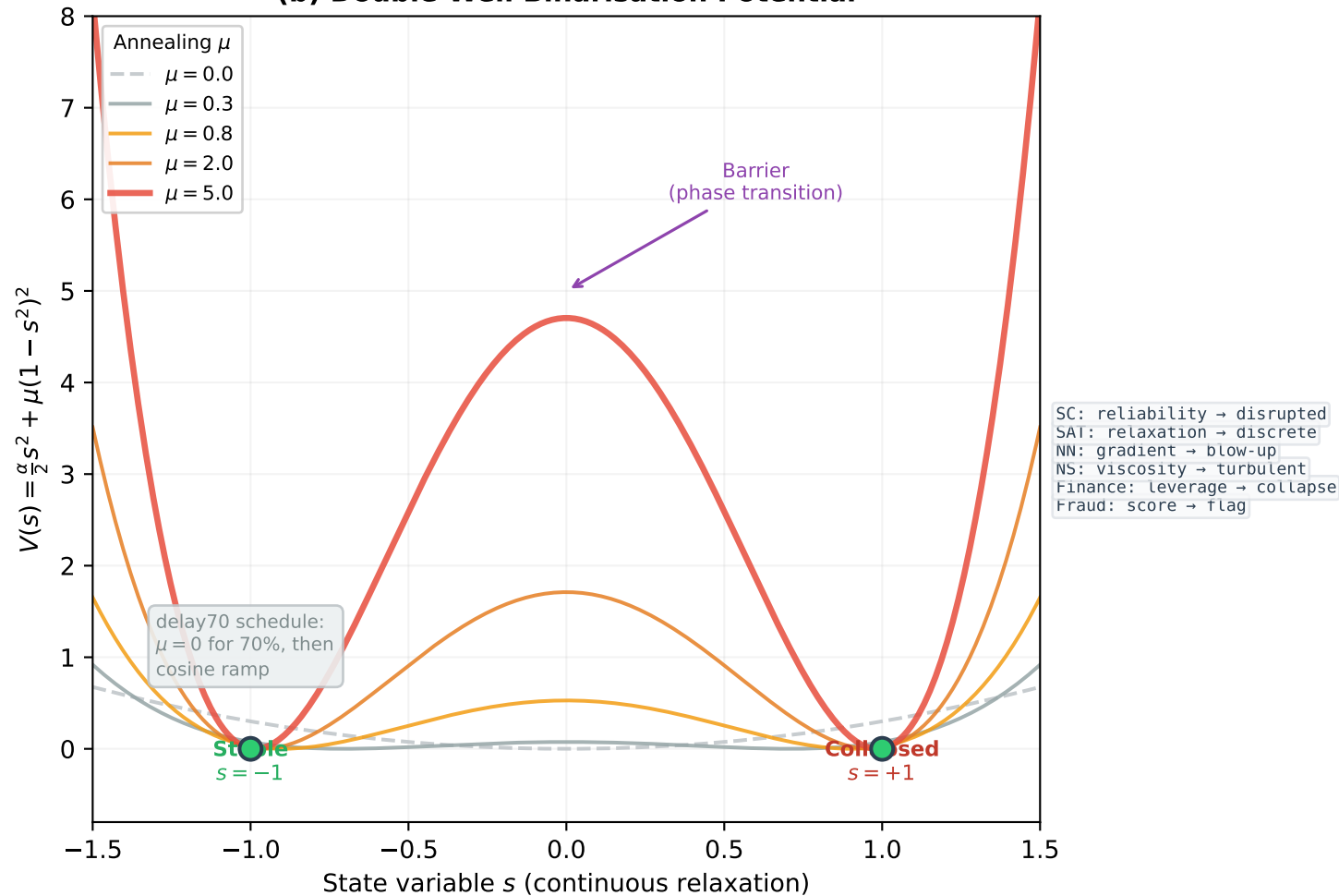
(b) Double-Well Binarisation Potential
