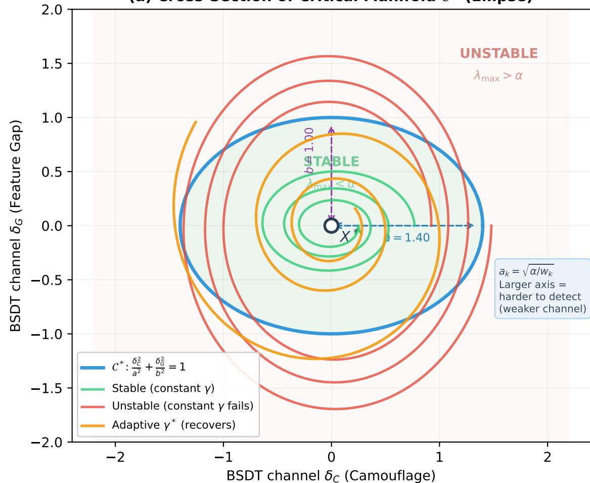
(a) Cross-Section of Critical Manifold \mathcal{C}^* (Ellipse)
