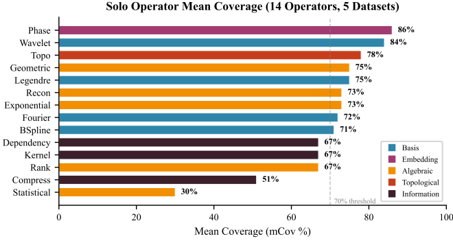
Fig. 3: Solo operator mean coverage across five datasets. Operators are ranked by mCov and colour-coded by mathematical family. Phase-curve (86%) and topological persistence (78%) lead; statistical and compression operators fall below the 70% utility threshold. No single operator exceeds 86%, confirming that multi-operator fusion is necessary.
