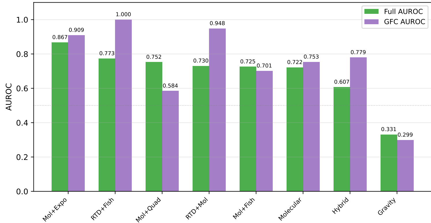
Algorithm Ranking: Full AUROC vs GFC-Window AUROC
