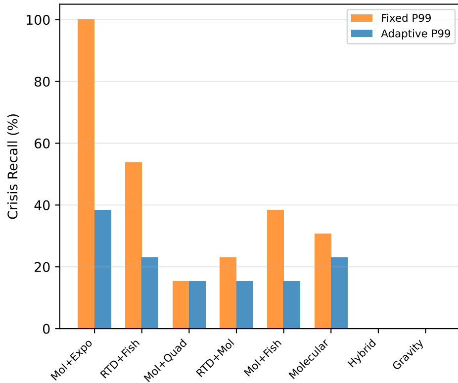
Recall: Fixed vs Adaptive
