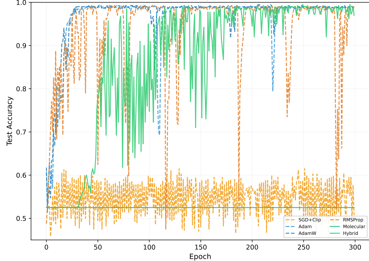
(b) Test Accuracy Comparison
