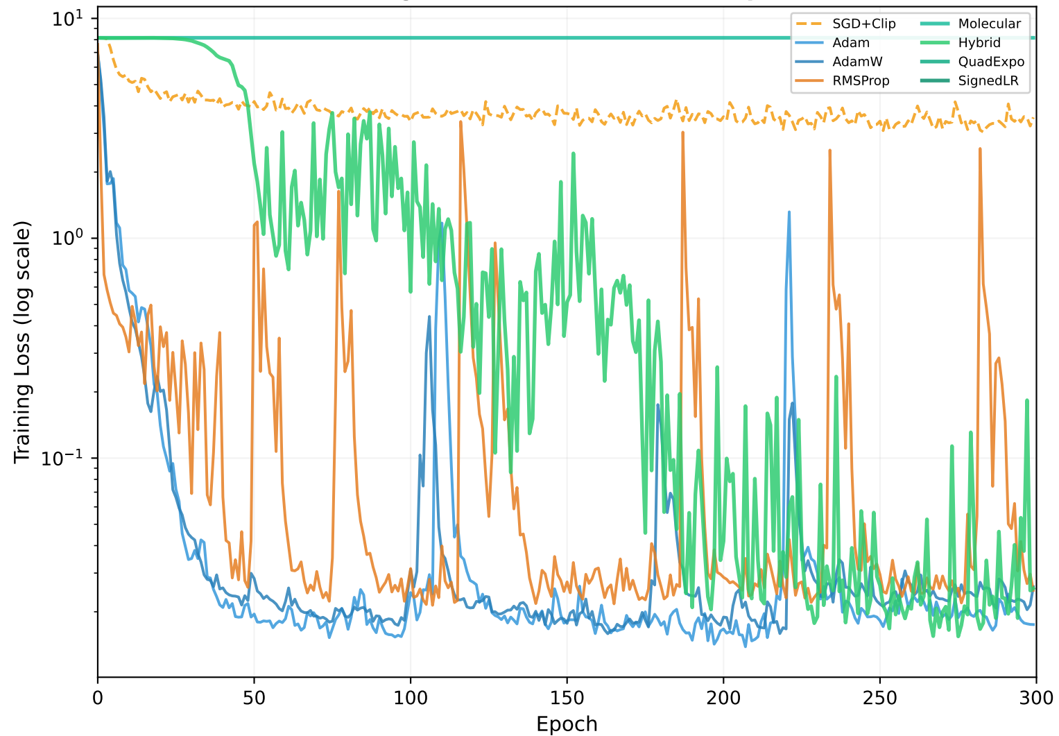
(a) Training Loss: Standard vs BSDT Optimisers
