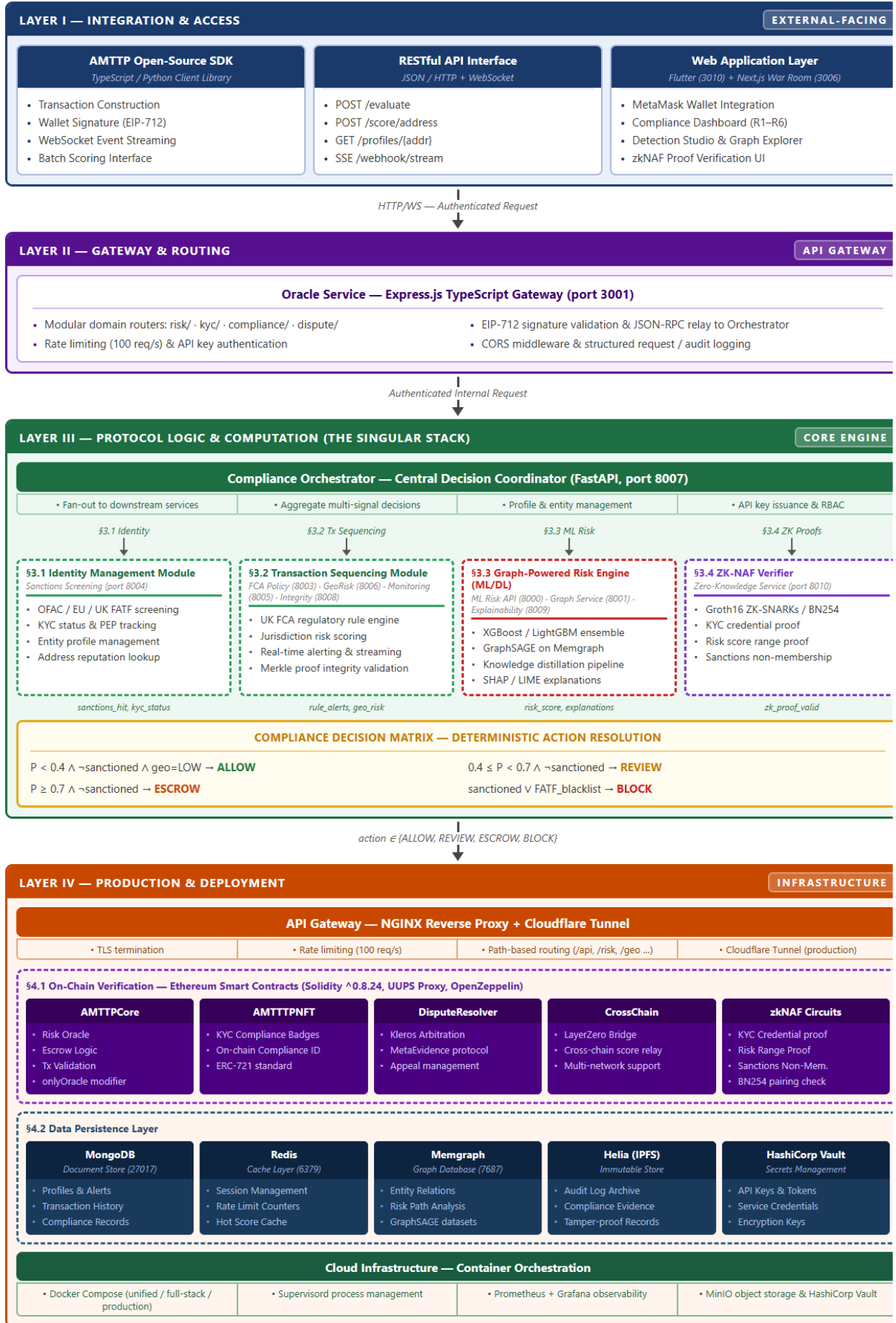
Figure 2: AMTTP four-layer architecture — Flutter + Next.js (UI) → Express Gateway → Python FastAPI orchestrator (9 microservices) → 5 upgradeable Solidity contracts, 17 Docker containers. All layers sole-authored.
