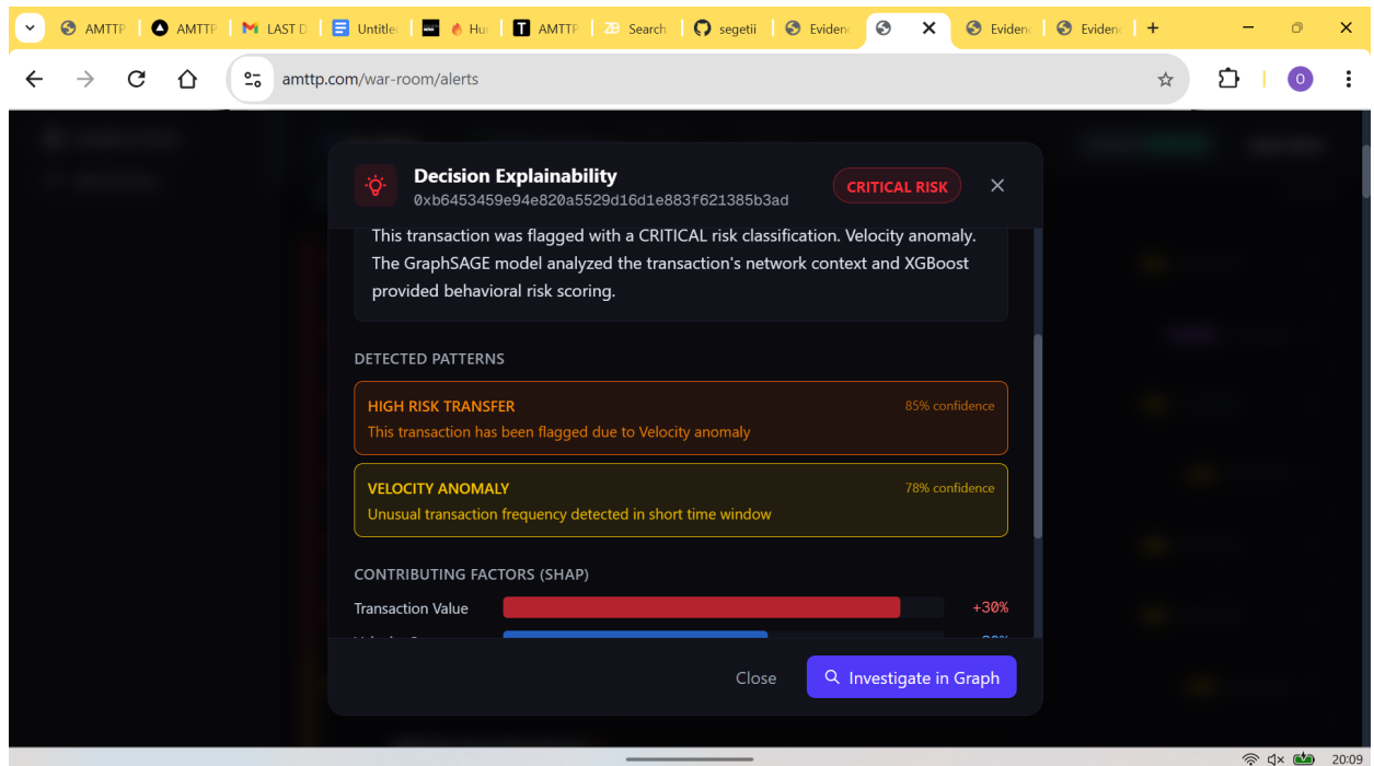
Figure 4: Decision Explainability panel for a CRITICAL alert — contributing factors and their weights: High Risk Transfer 85%, Velocity Anomaly 78%, Sanctioned Address Proximity 65%, with direct link to the graph network view. Satisfies FCA/MiCA audit trail requirements without additional tooling.
