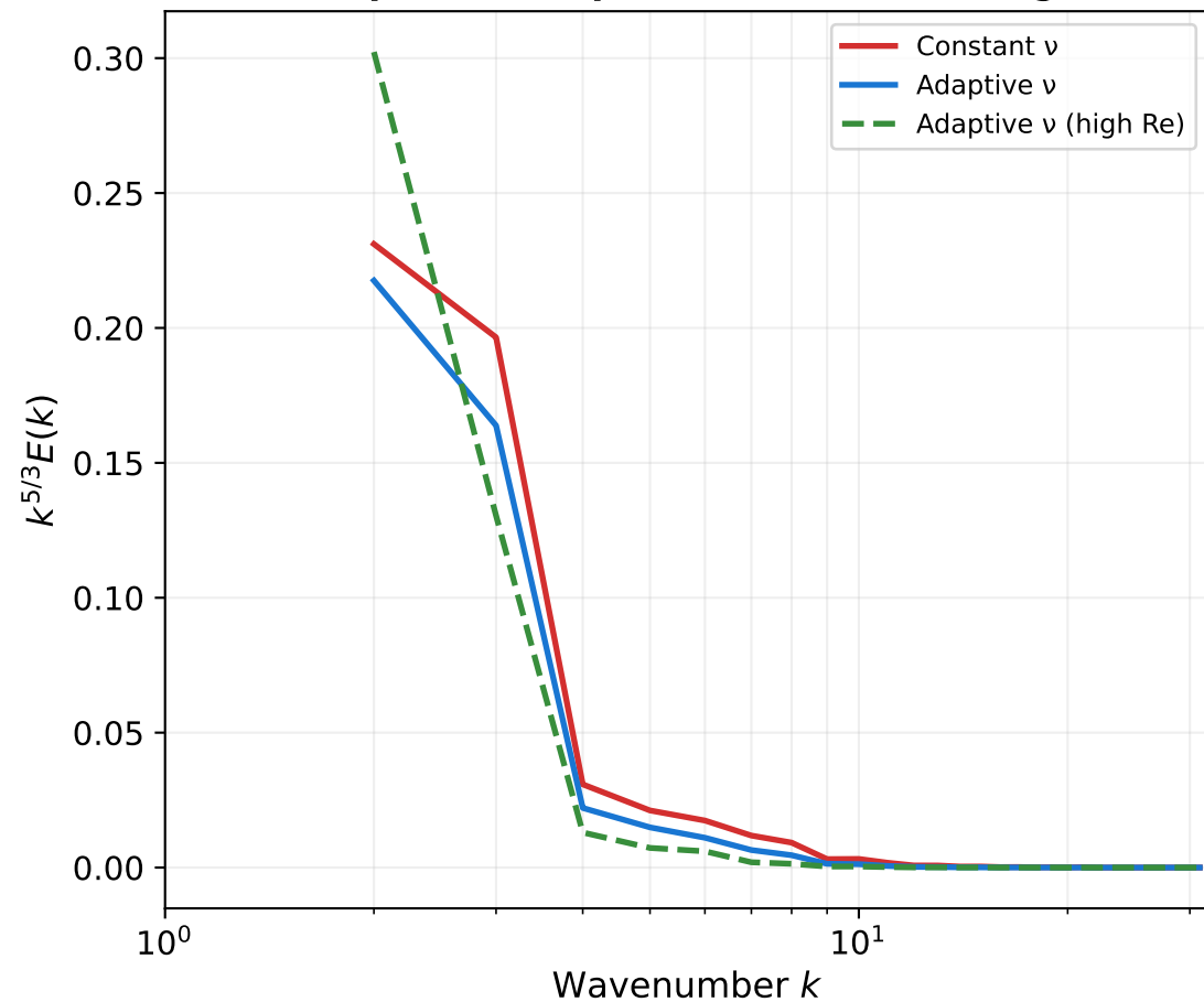
(b) Compensated Spectrum (flat = Kolmogorov)
