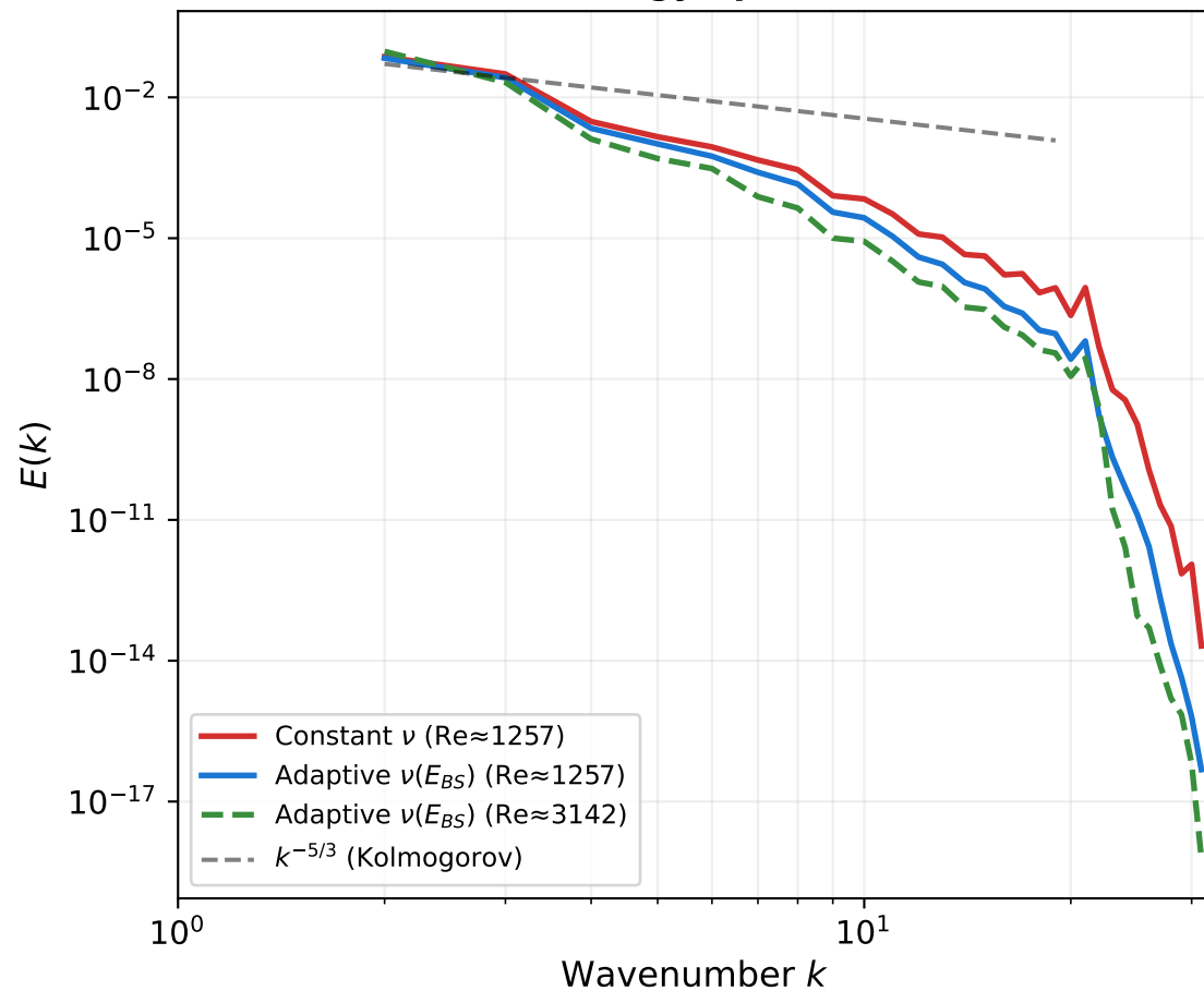
(a) Energy Spectrum
