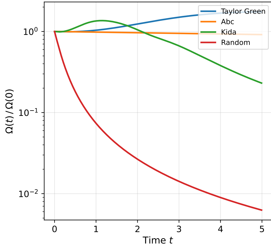
(a) Normalised Enstrophy — All ICs
