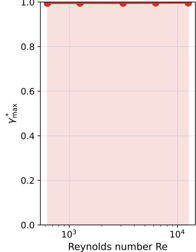
(c) Peak Adaptive Damping \gamma^*
