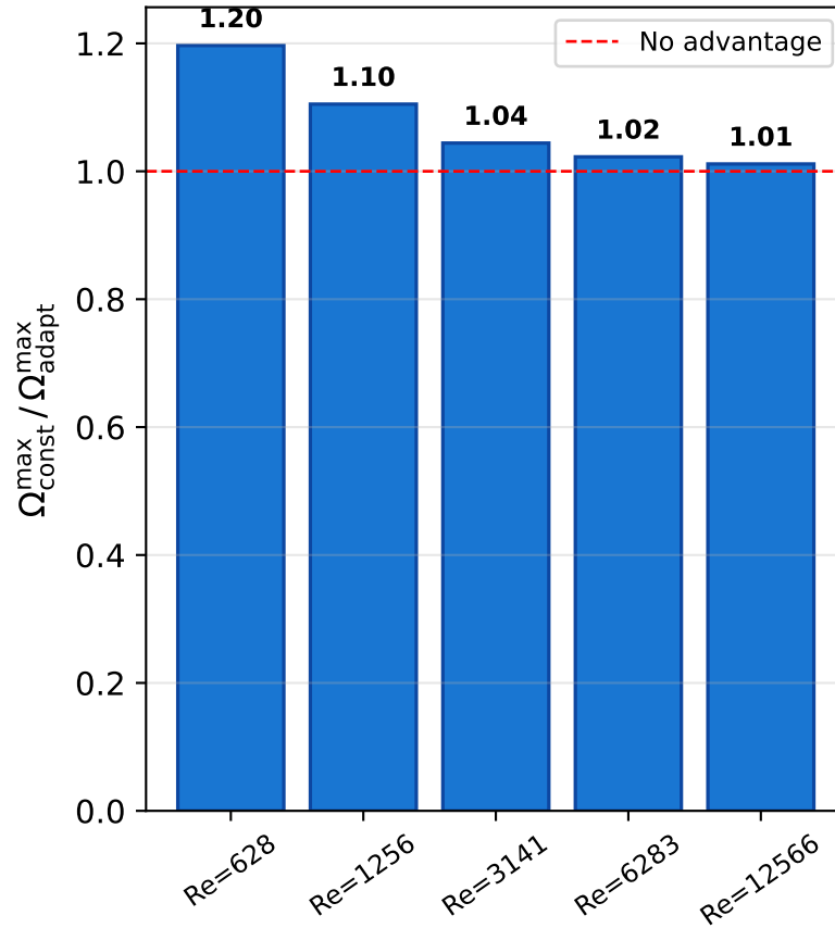
(b) Enstrophy Suppression Factor
