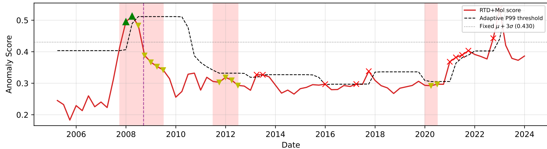
RTD+Mol (AUROC = 0.730)
