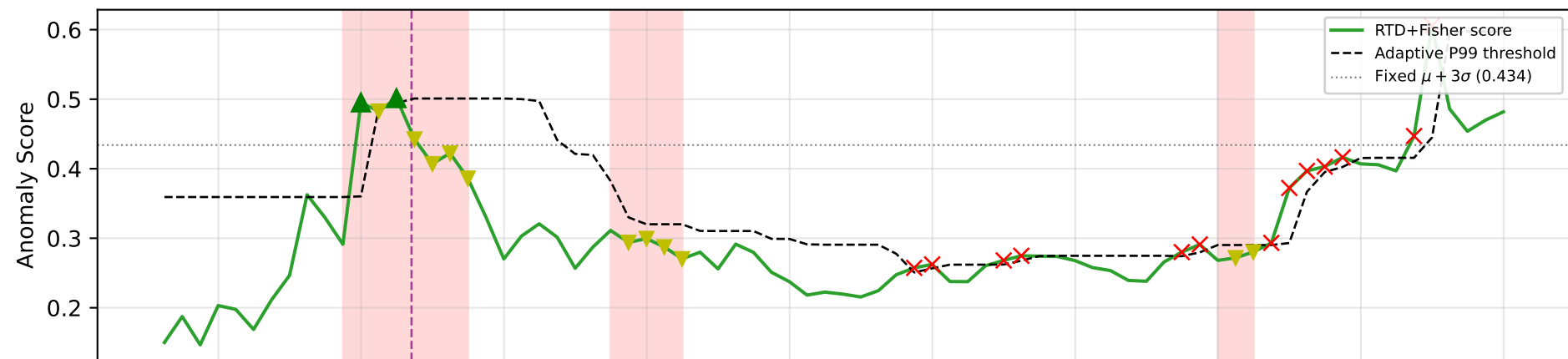
RTD+Fisher (AUROC = 0.773)
