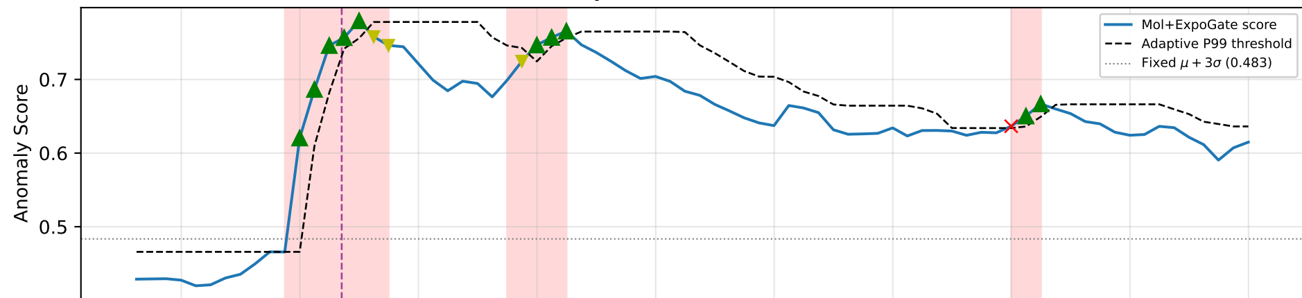
Mol+ExpoGate (AUROC = 0.867)
