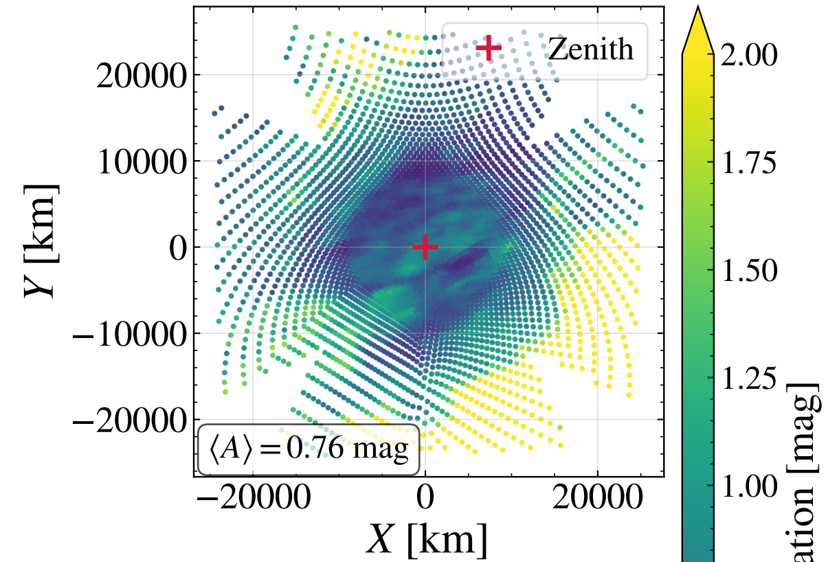
Flat Sky (X, Y)
