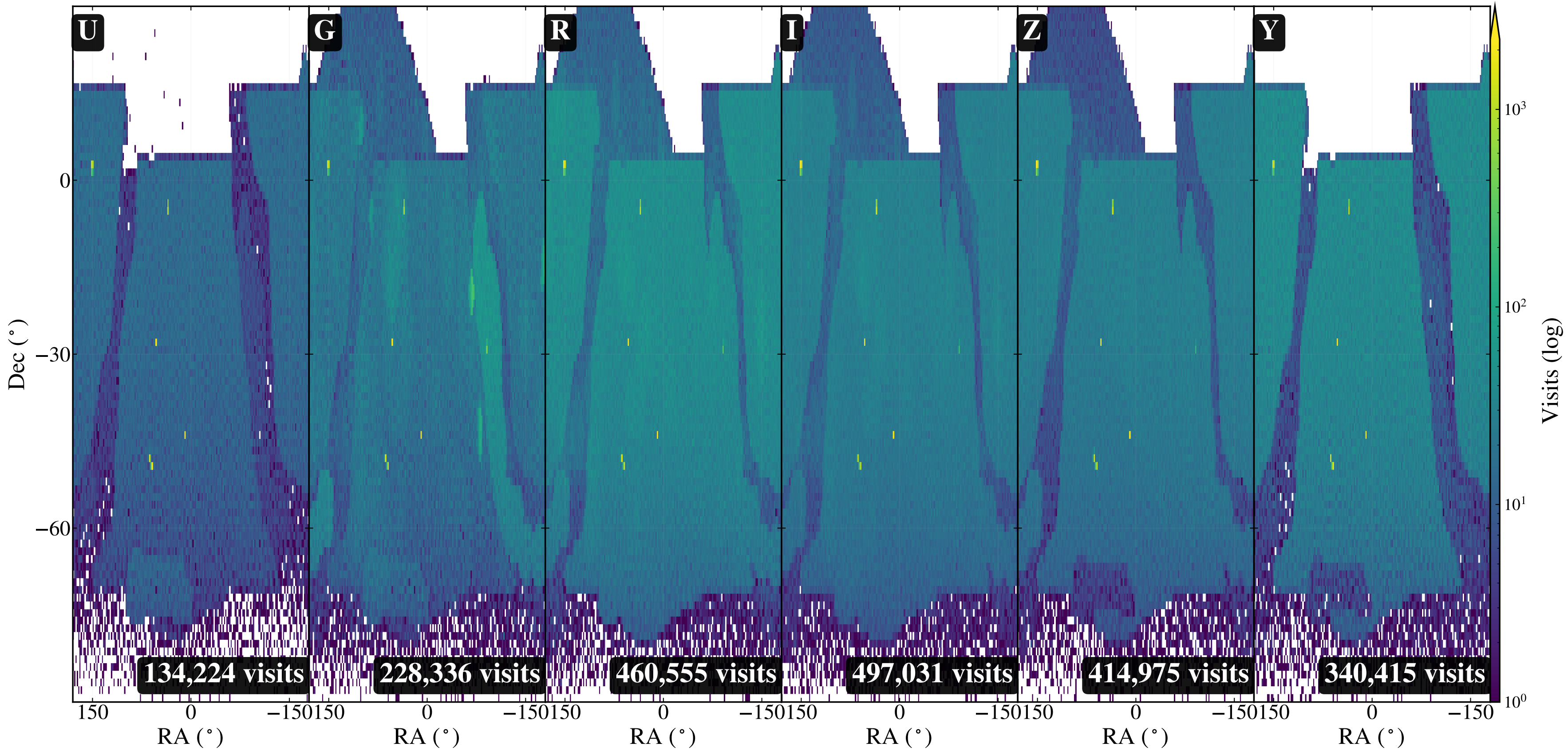
LSST 10-Year Sky Coverage by Filter
