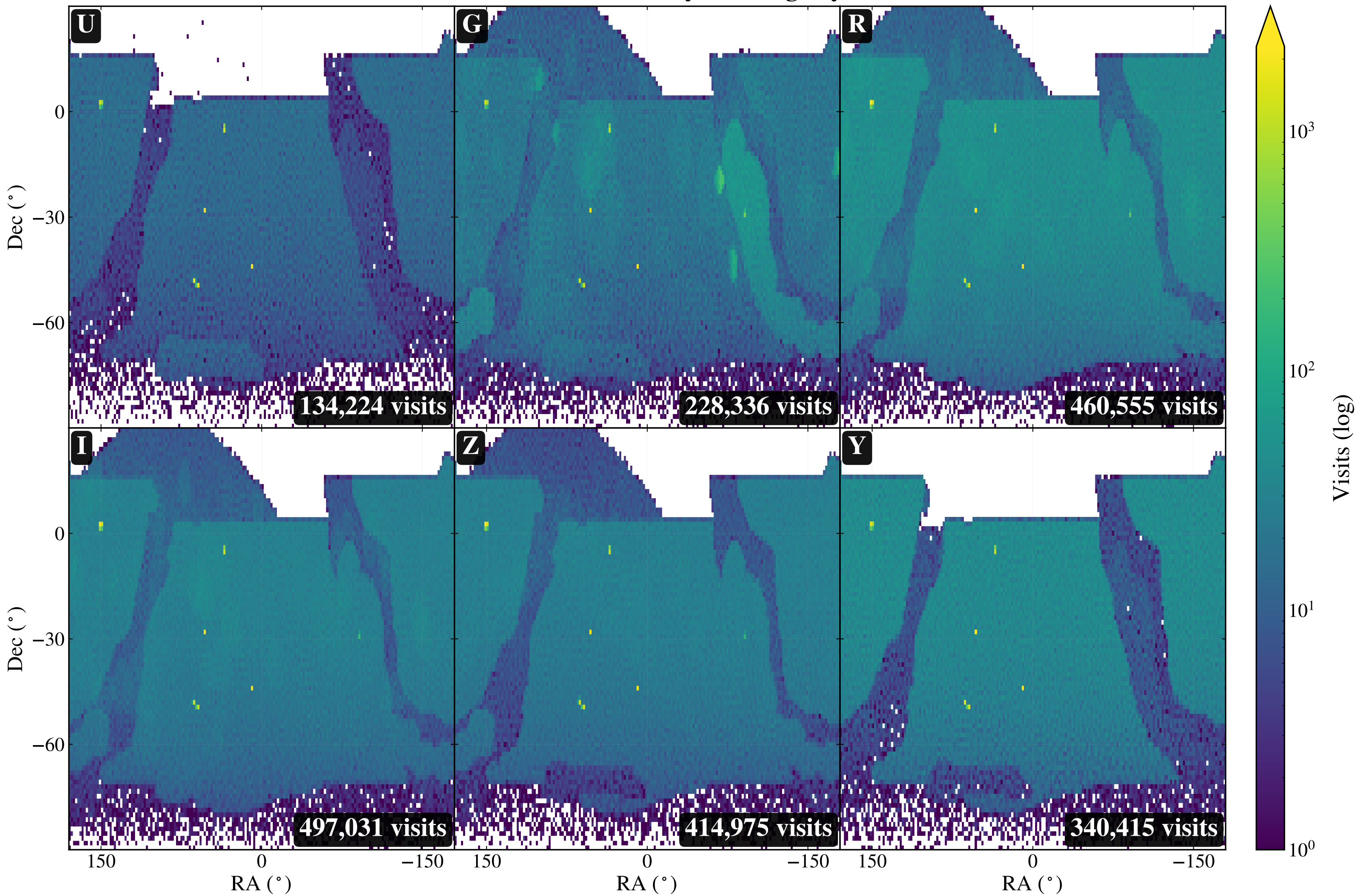
LSST 10-Year Sky Coverage by Filter
