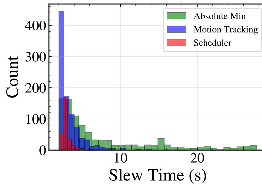
Slew Time Distribution
