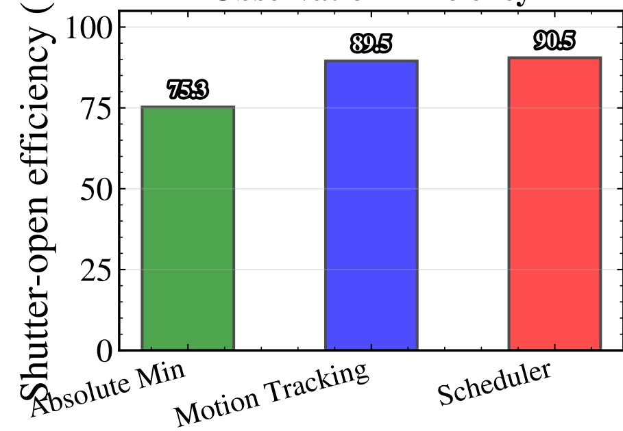
Observation Efficiency
