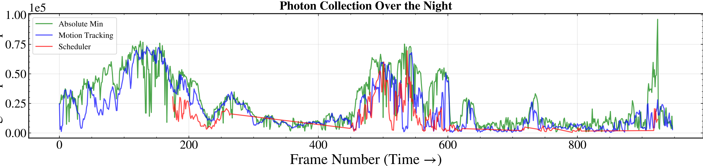
Total Night Photon Collection
