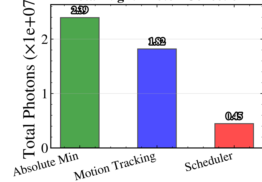
Total Night Photon Collection
