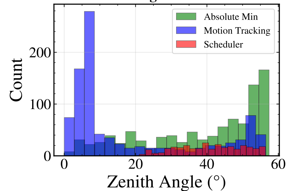
Zenith Angle Distribution
