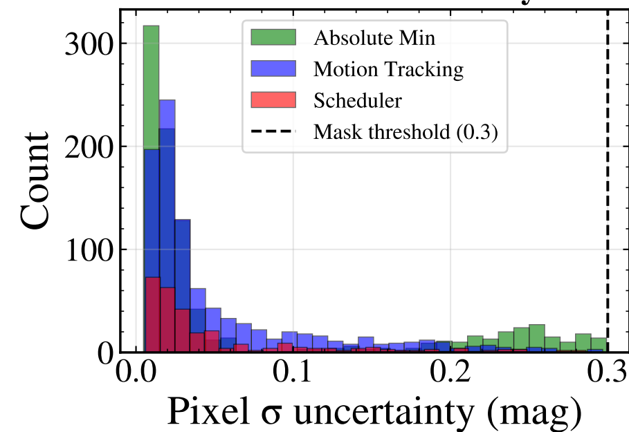
Extinction Uncertainty
