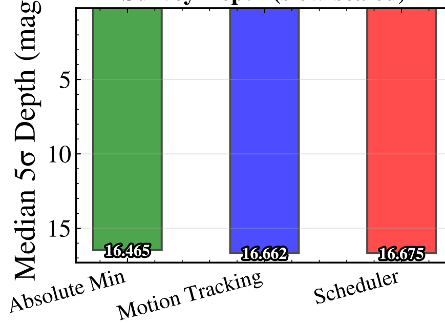
Survey Depth (slew-scaled)
