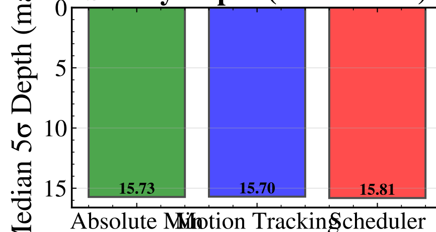
Survey Depth (slew-scaled)
