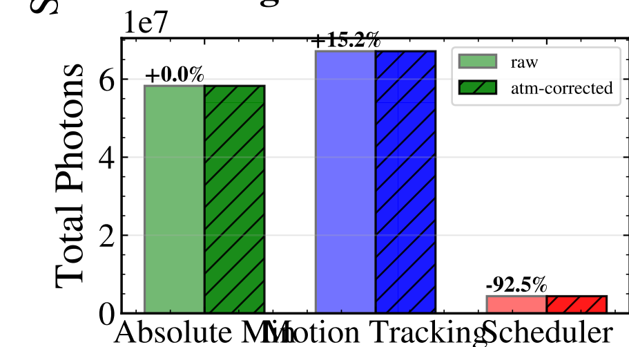
Total Night Photon Collection
