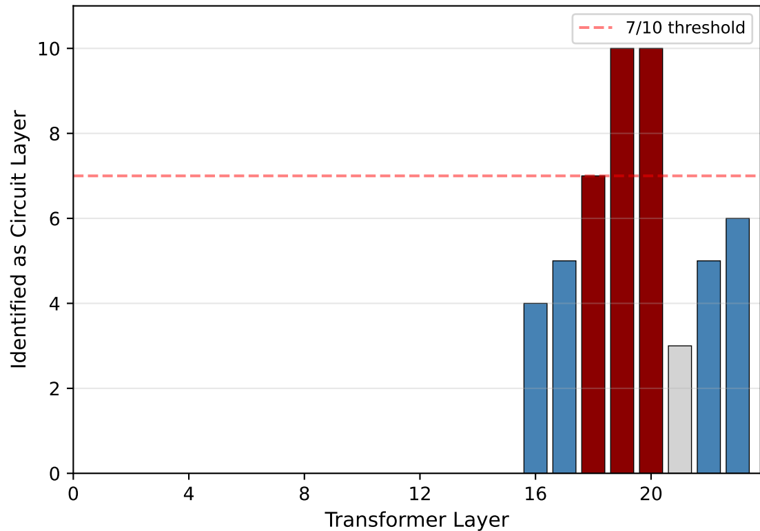
(b) Circuit Layer Identification (10 runs)
