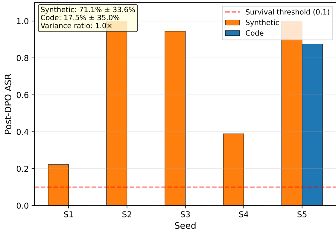
(b) Per-Seed DPO Residual ASR
